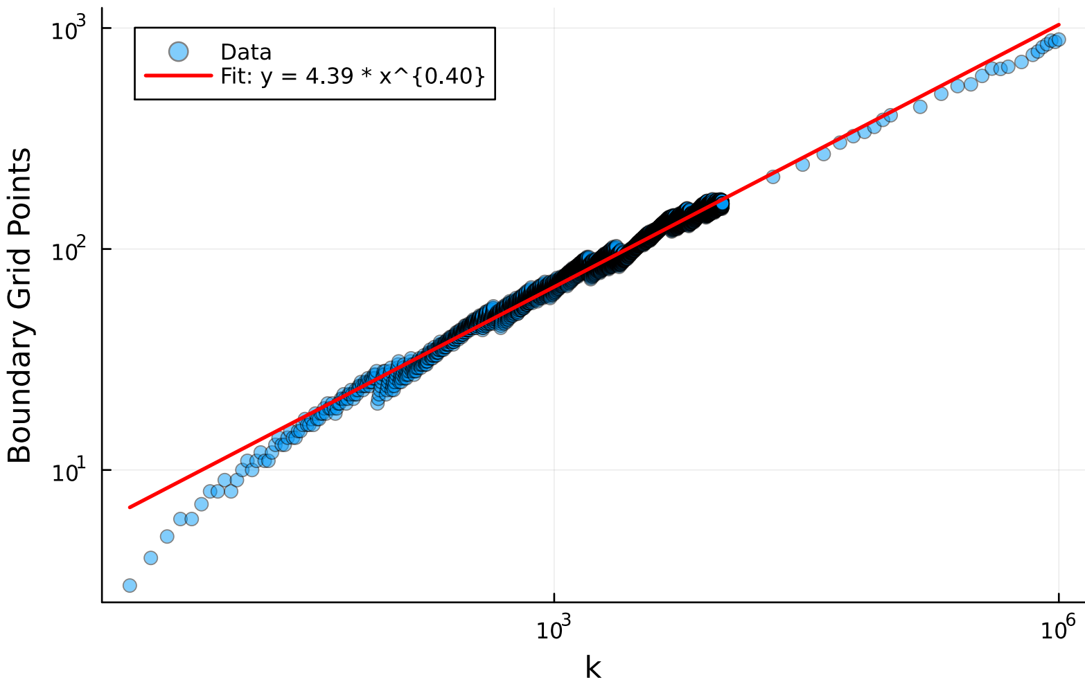
Log-Log Plot: Boundary Grid Points vs k
