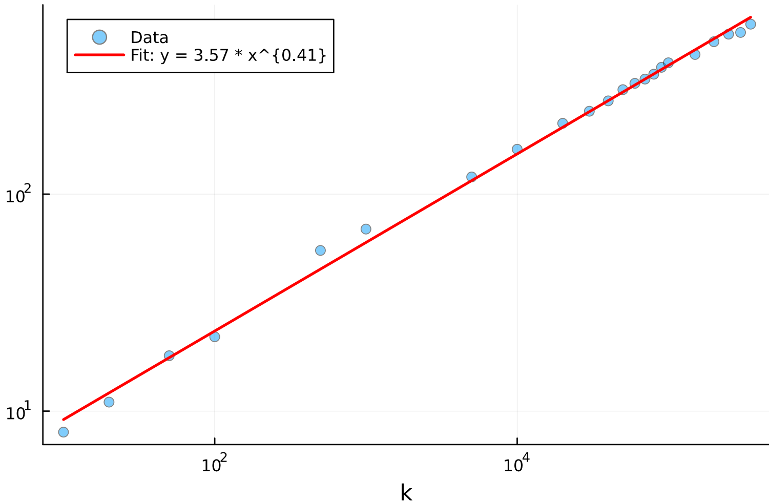
Log-Log Plot: Boundary Grid Points vs k
