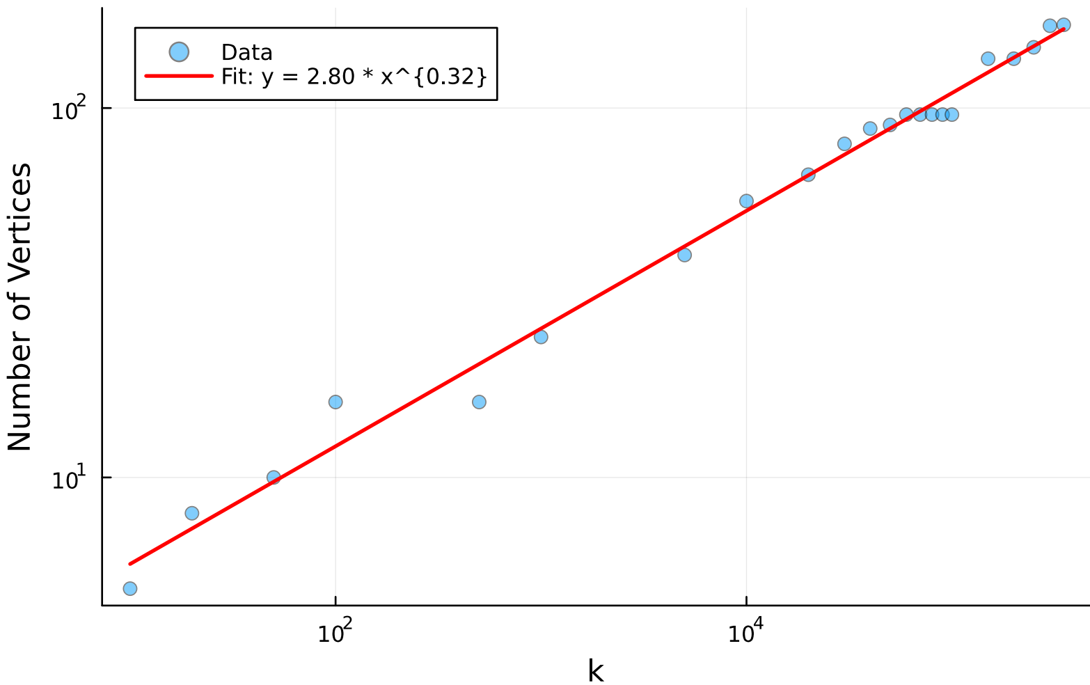
Log-Log Plot: Number of Vertices vs k
