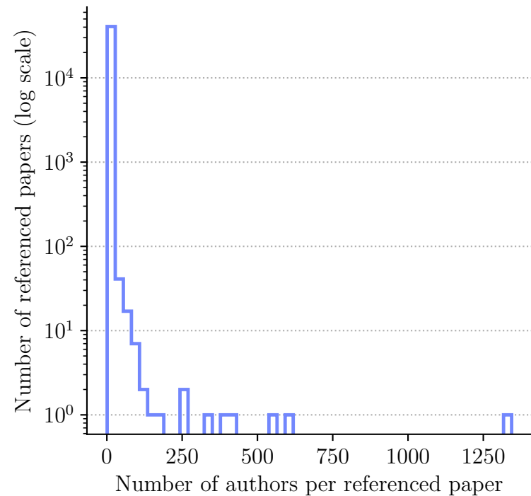
Author count distribution
