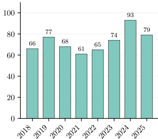
POPL
