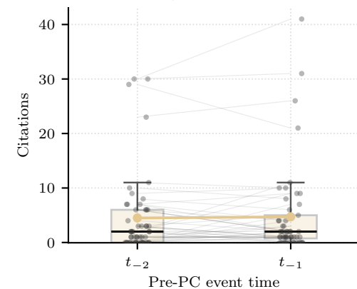
Pre-PC raw citations mean: t_{-2} 4.5; t_{-1} 4.7
