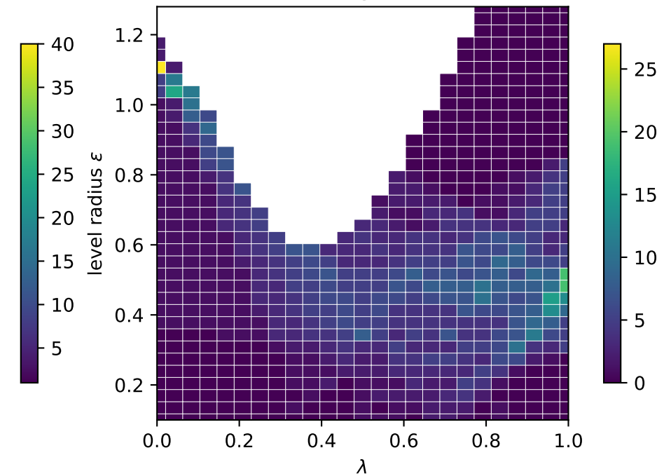
total genus
