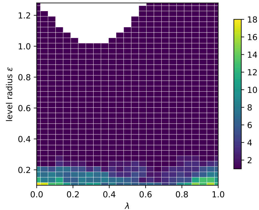
volume components
