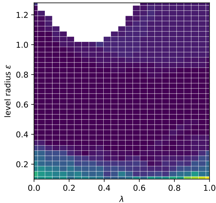
surface components
