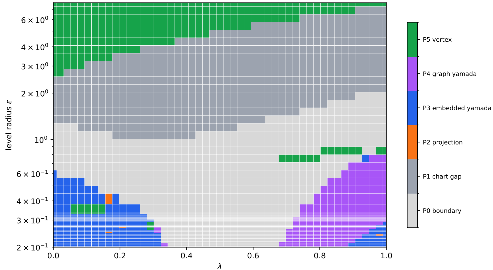
Trefoil to figure-eight compactified Yamada certification overview
