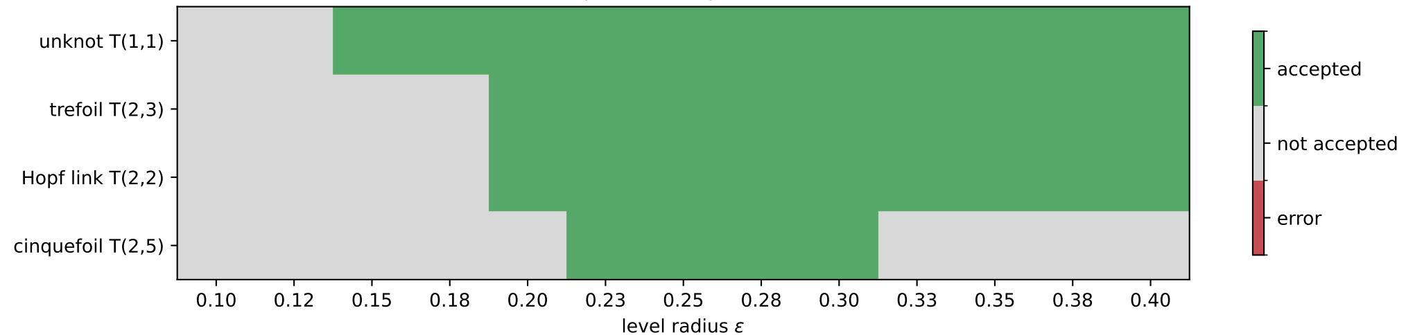
Static knot/link epsilon acceptance at dimension 96
