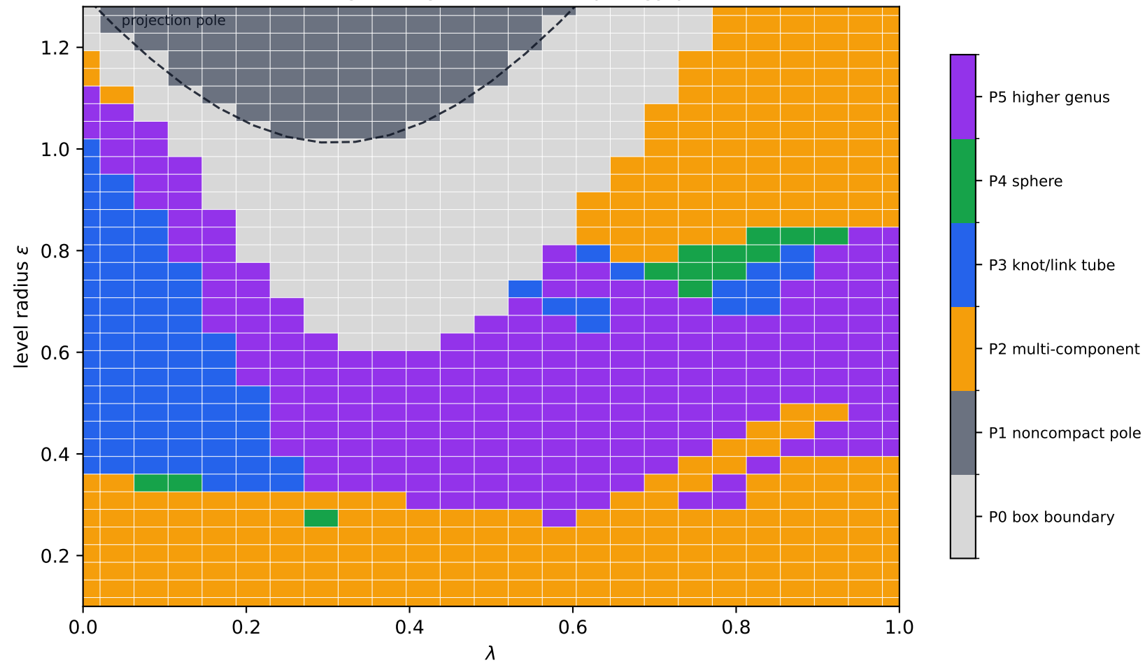
Trefoil to figure-eight level-set topology phases
