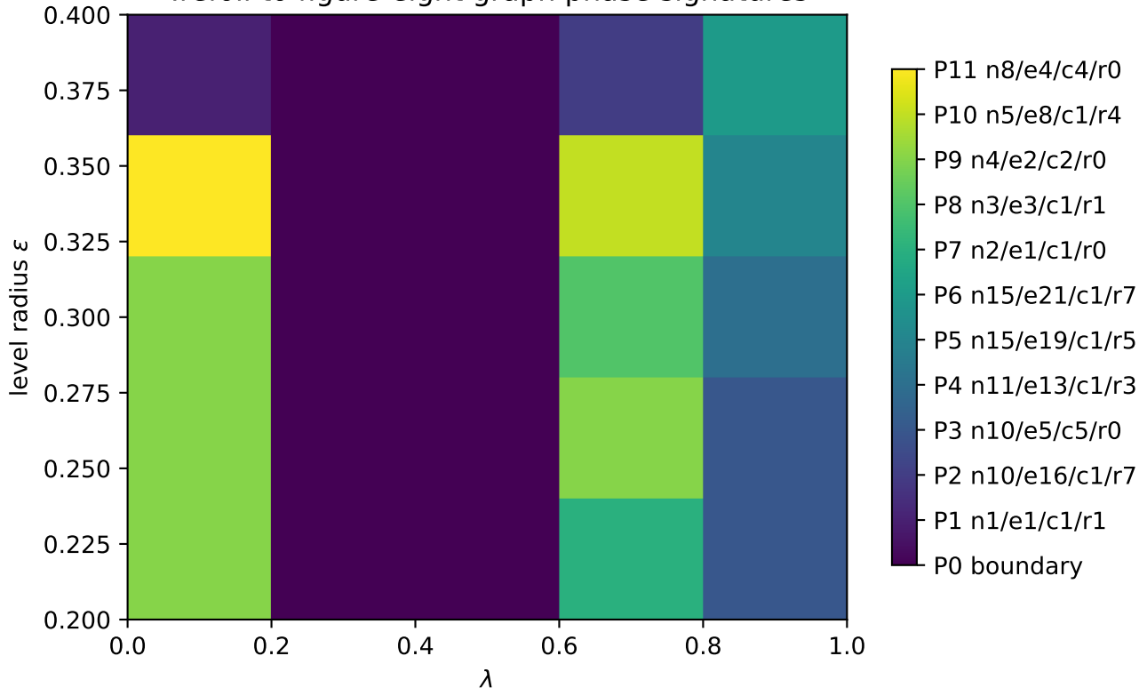
Trefoil to figure-eight graph phase signatures
