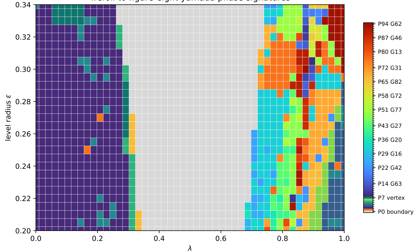
Trefoil to figure-eight yamada phase signatures
