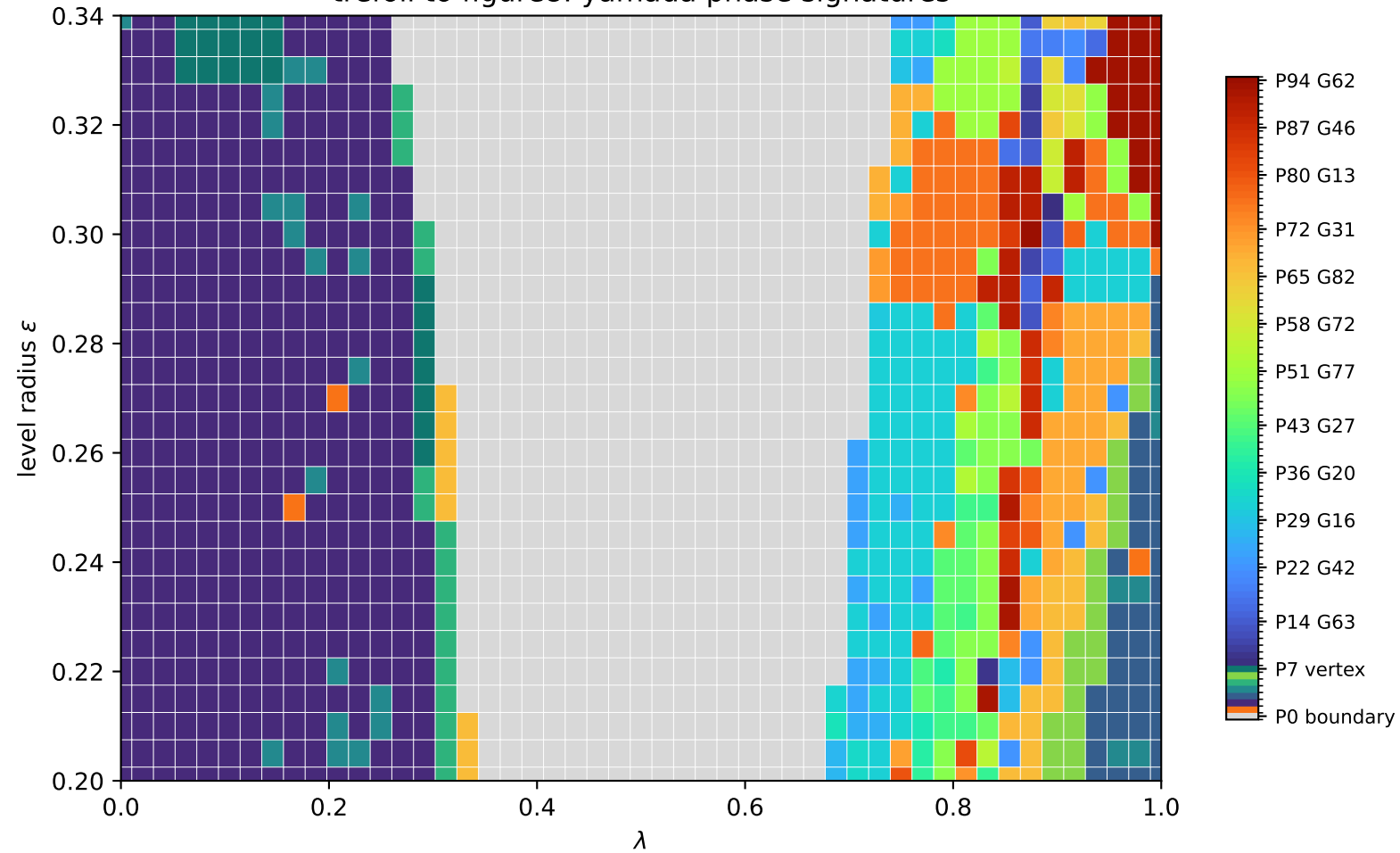
trefoil to figure8: yamada phase signatures
