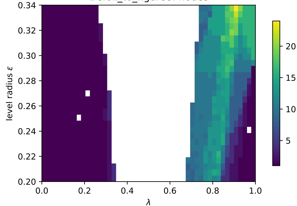
trefoil_to_figure8: nodes
