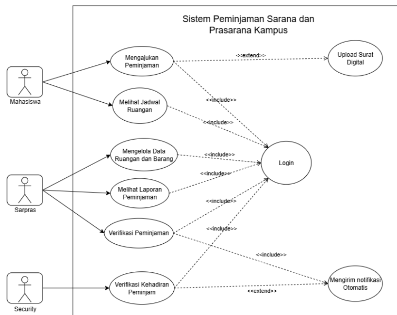
Figure 3.2: Usecase Diagram
