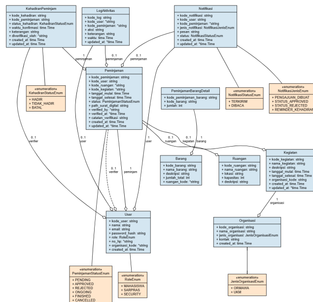
Gambar 3.10: Class Diagram
