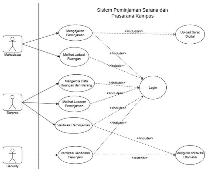
Gambar 3.2: Usecase Diagram
