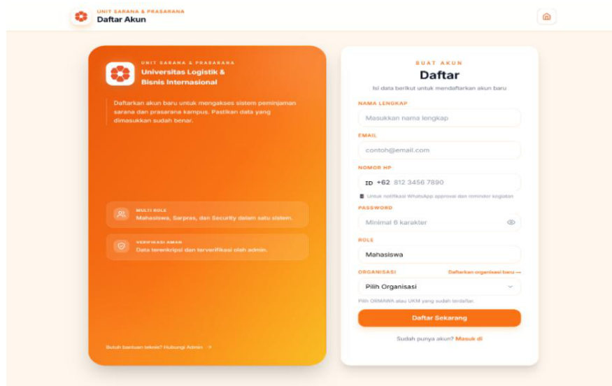
Gambar 4.3: Halaman Register
