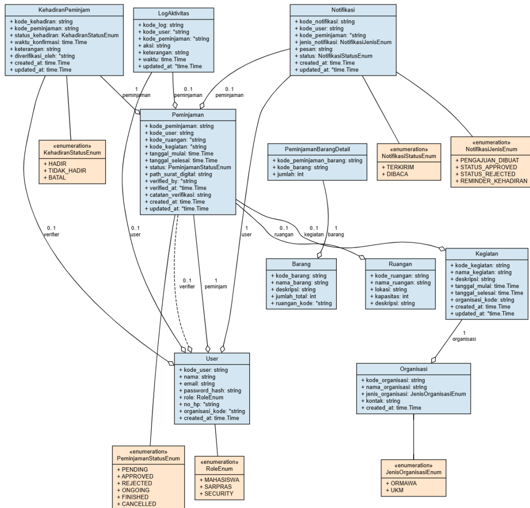
Gambar 3.10: Class Diagram
