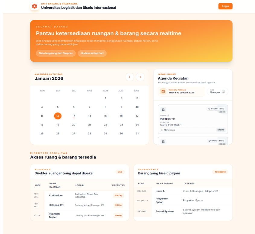
Figure 4.1: Halaman Utama
