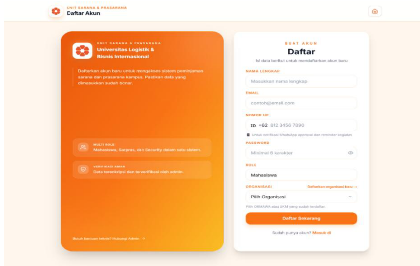
Figure 4.3: Halaman Register
