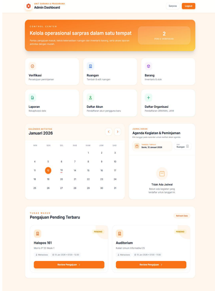
Figure 4.6: Dashboard Sarpras
