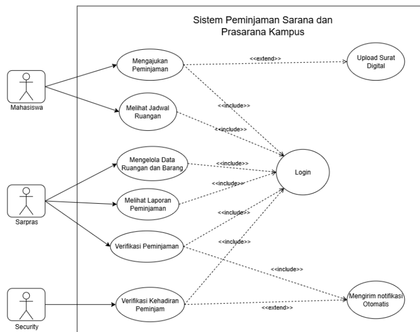
Figure 3.2: Usecase Diagram
