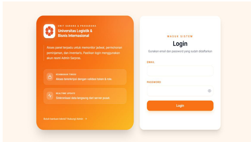
Figure 4.2: Halaman Login
