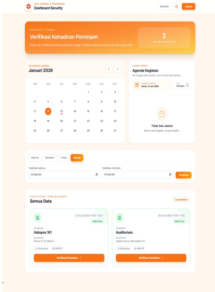
Figure 4.9: Dashboard Security
