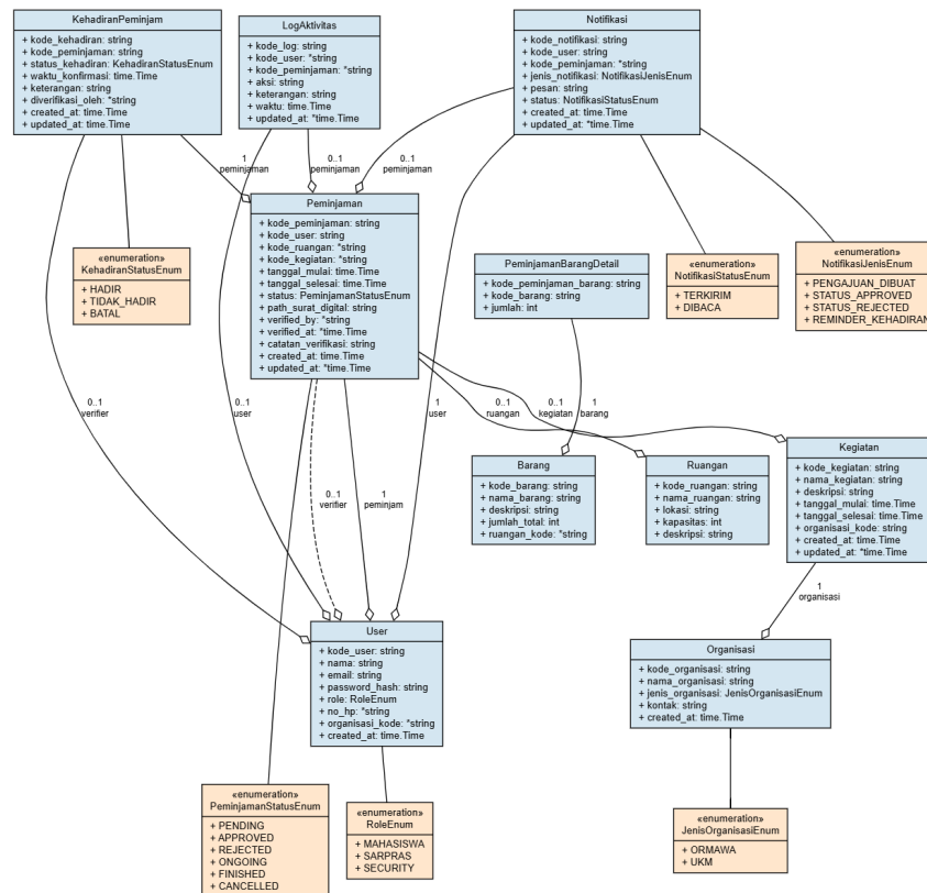
Figure 3.10: Class Diagram
