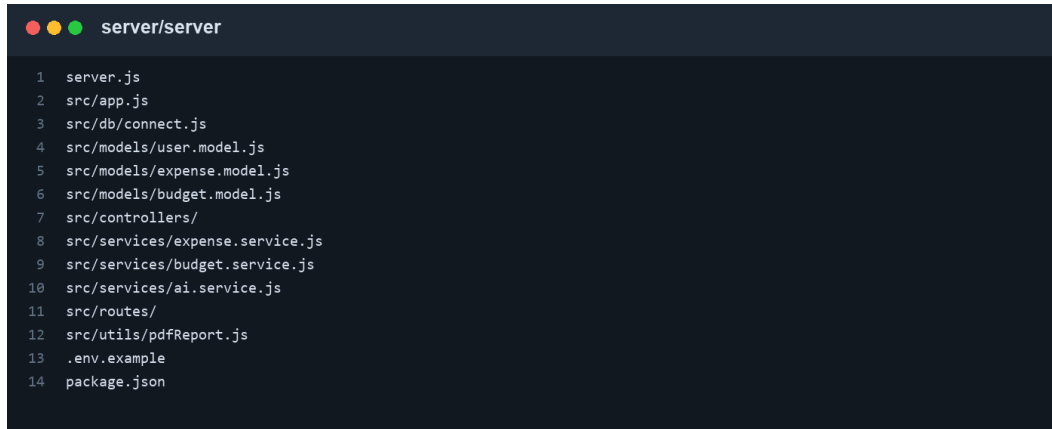
Figure 5. Backend project structure
