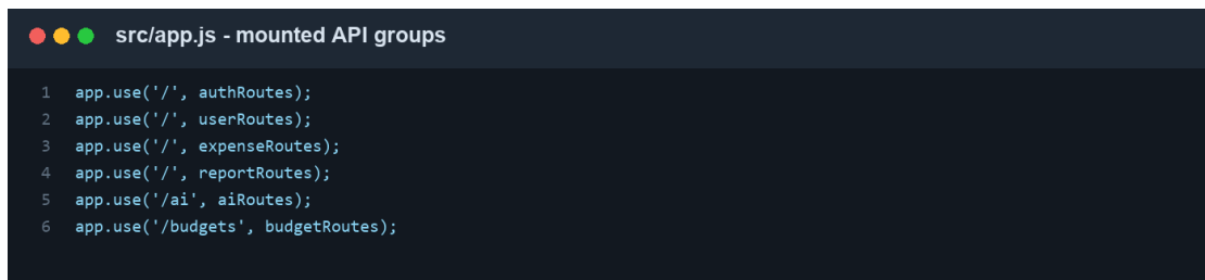
Figure 6. Route groups mounted by the Express application
