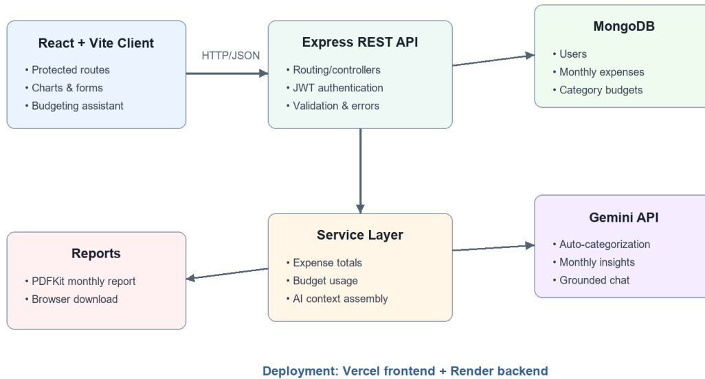
Figure 1. FinGPT technical architecture
