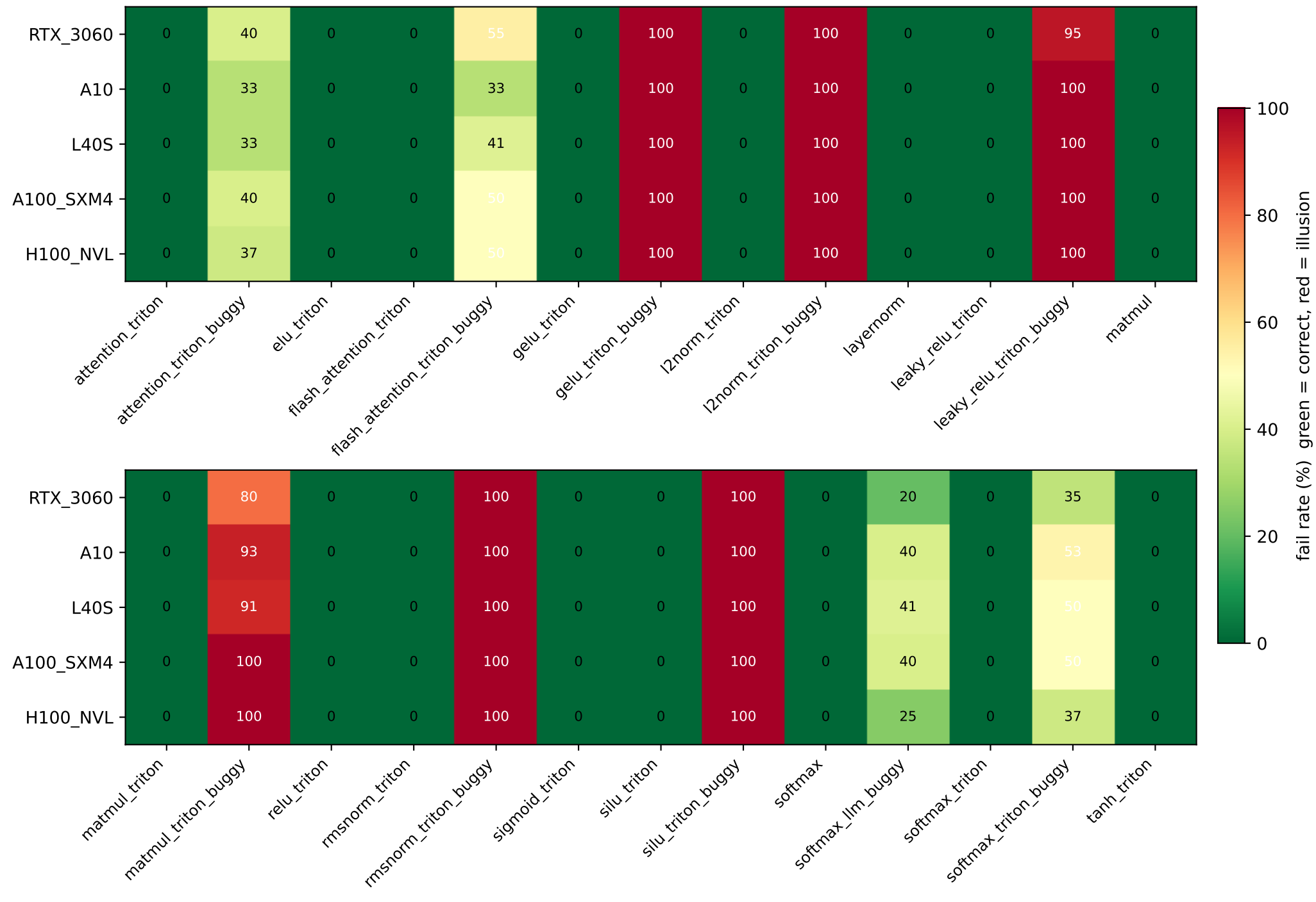
P1: cross-GPU verdict consistency on the 26-op corpus
