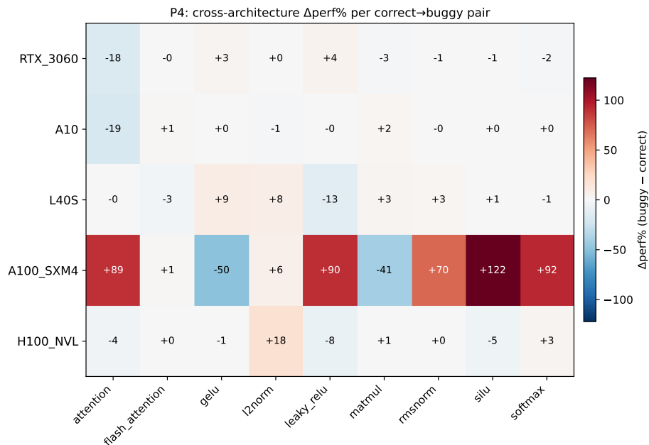
Fig. 2. Cross-architecture \Delta\text{perf}\% per pair. Only the measured signal varies; static \Delta is identical across all five GPUs.
