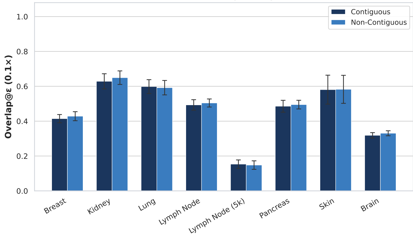
Overlap@ \epsilon (0.1x) by Query Pattern
