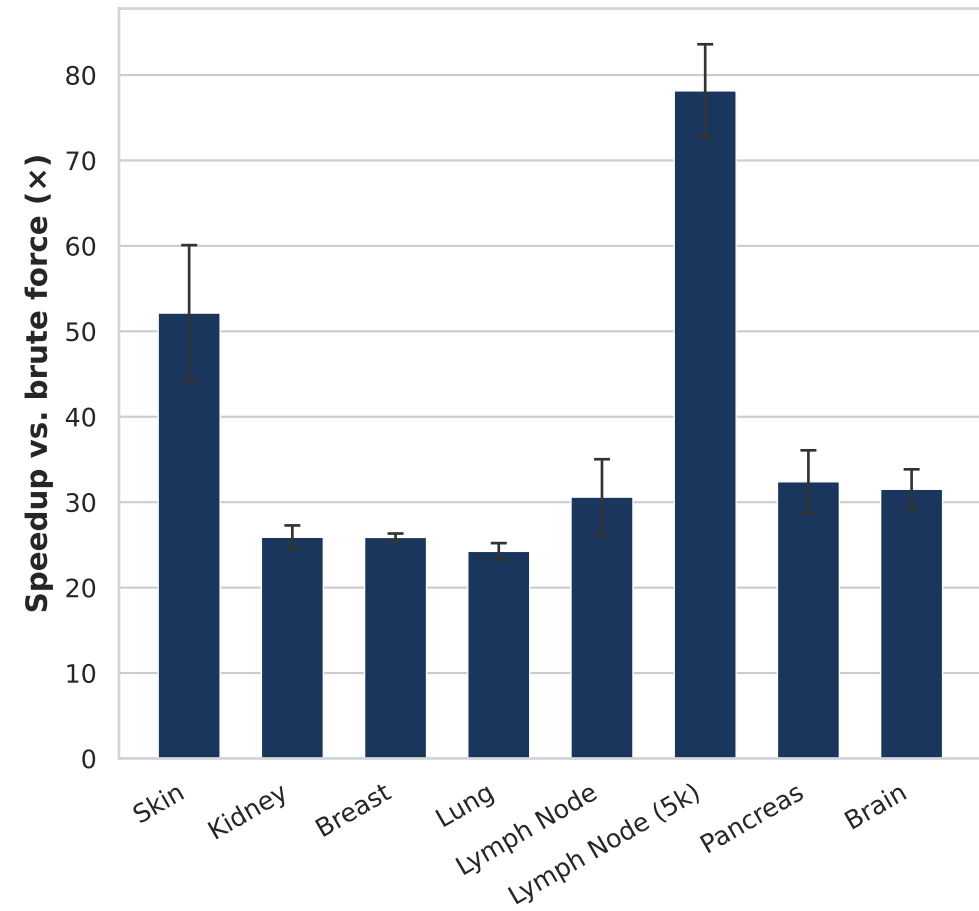
Mean speedup (mean \pm s.d., seeds 0-4)
