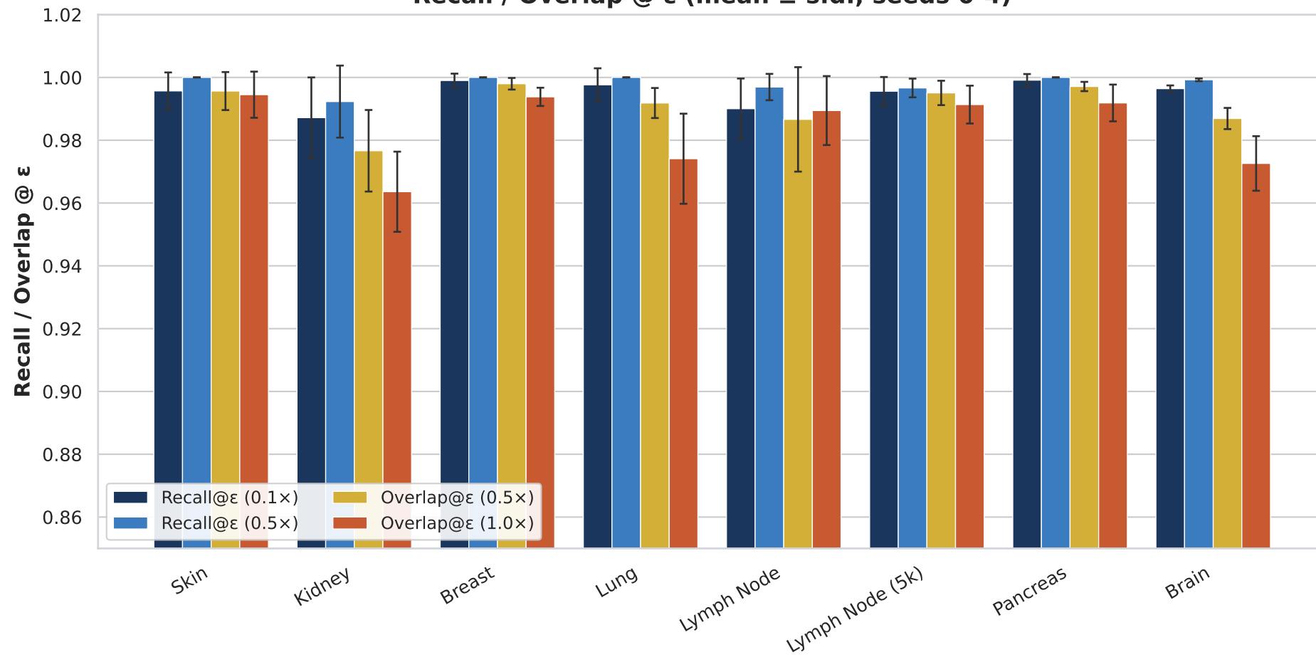
Recall / Overlap @ \epsilon (mean \pm s.d., seeds 0-4)
