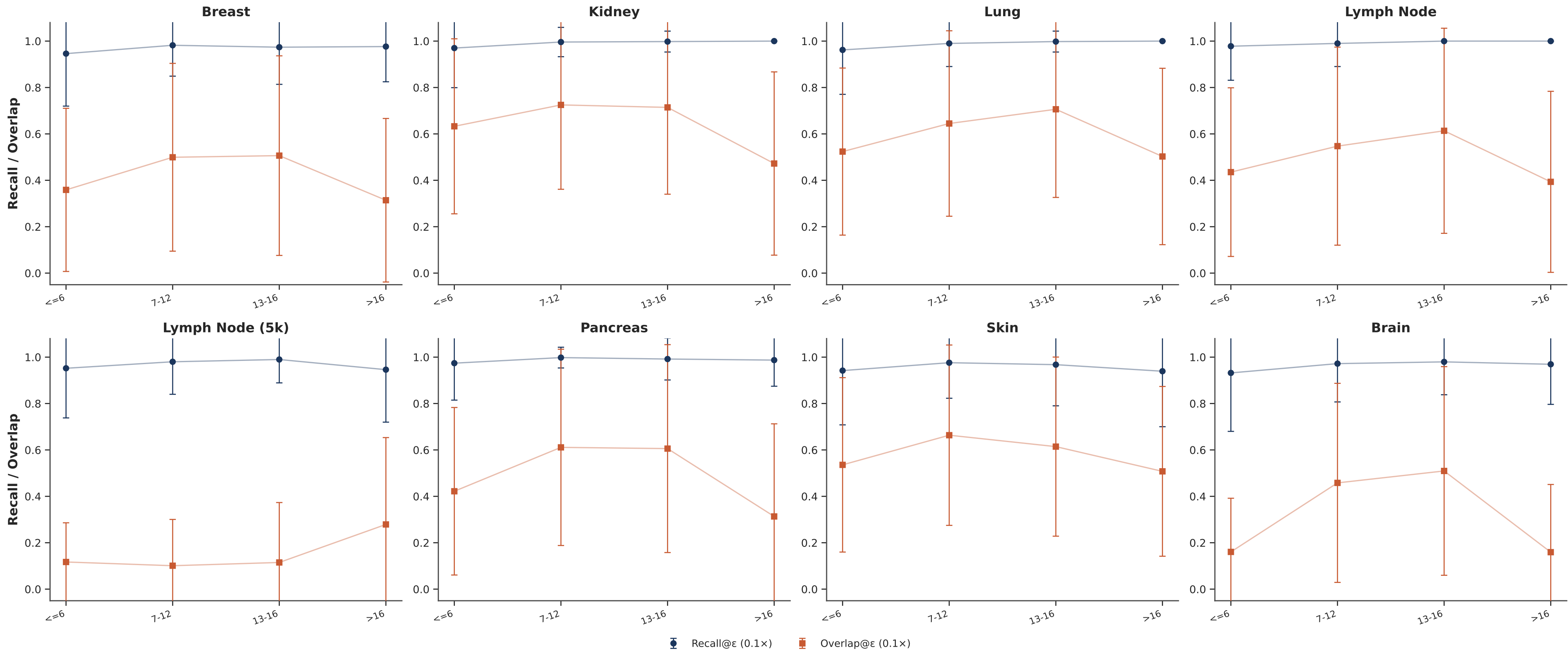
Partial-Panel-Search Accuracy vs. Query Length (mean \pm s.d., seeds 0-4)
