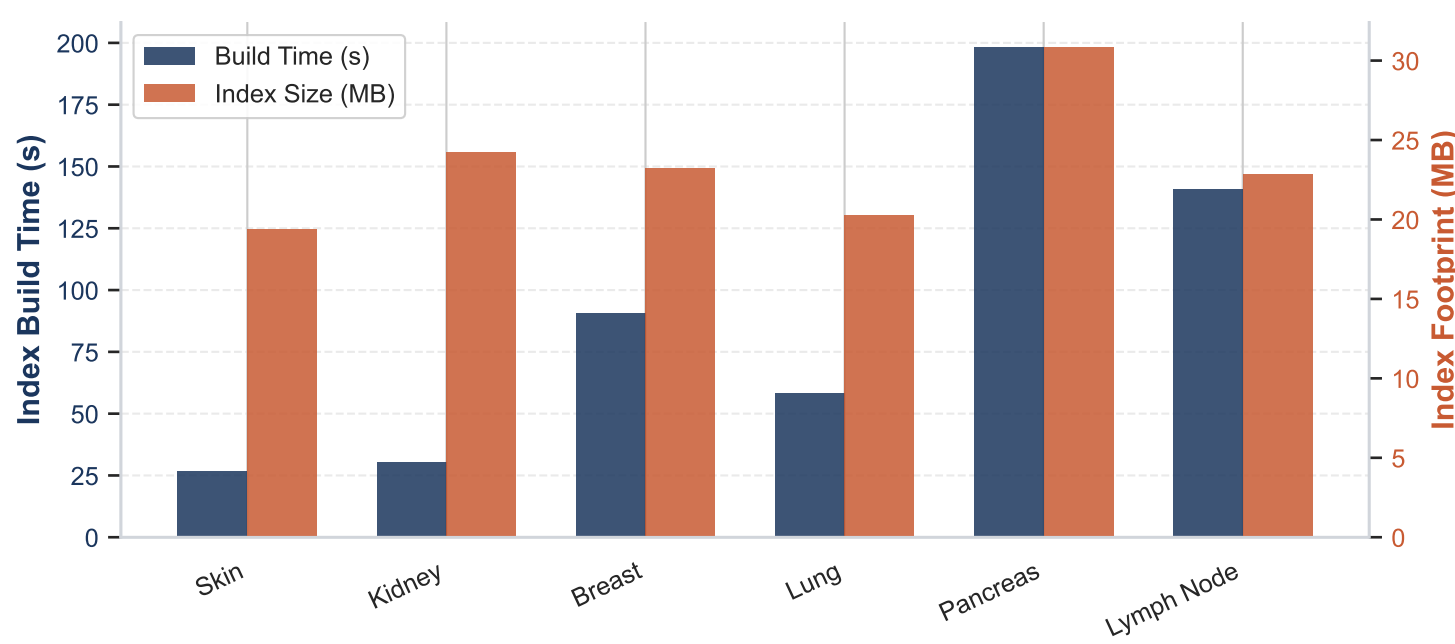
Figure 1: SPINDLE Core Architecture, Ultra-Fast Indexing, and Spatial Search Performance Index Scalability & Memory Footprint (Sub-linear Build Time & Compact Storage)
