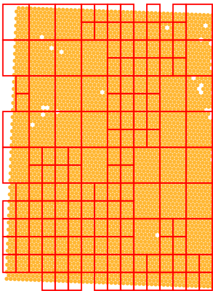
Visium (157 tiles)
