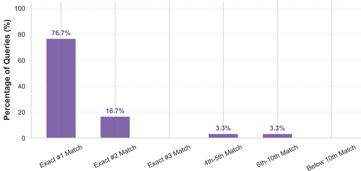
Accuracy of Spindle First Match (Percentage of queries where Spindle found the exact #1 best match, #2 best match, and so on)
