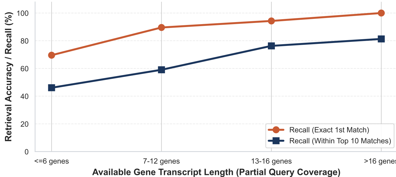
Partial Query Search Accuracy (High recall despite searching with incomplete or truncated gene transcripts)
