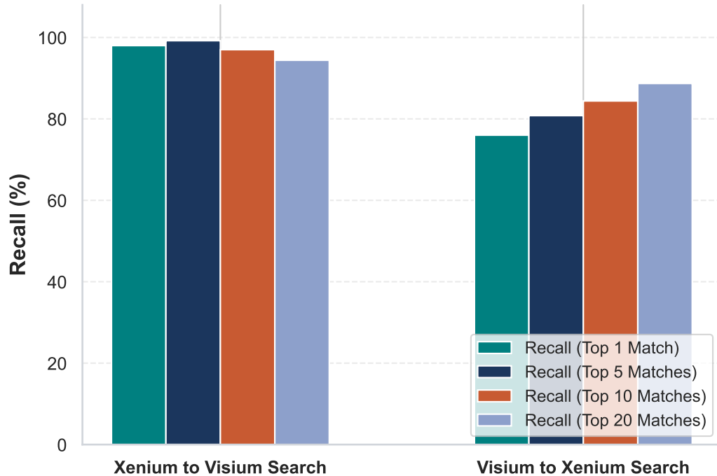
Cross-Modality Retrieval Accuracy (Percentage of true matches found within top candidates)
