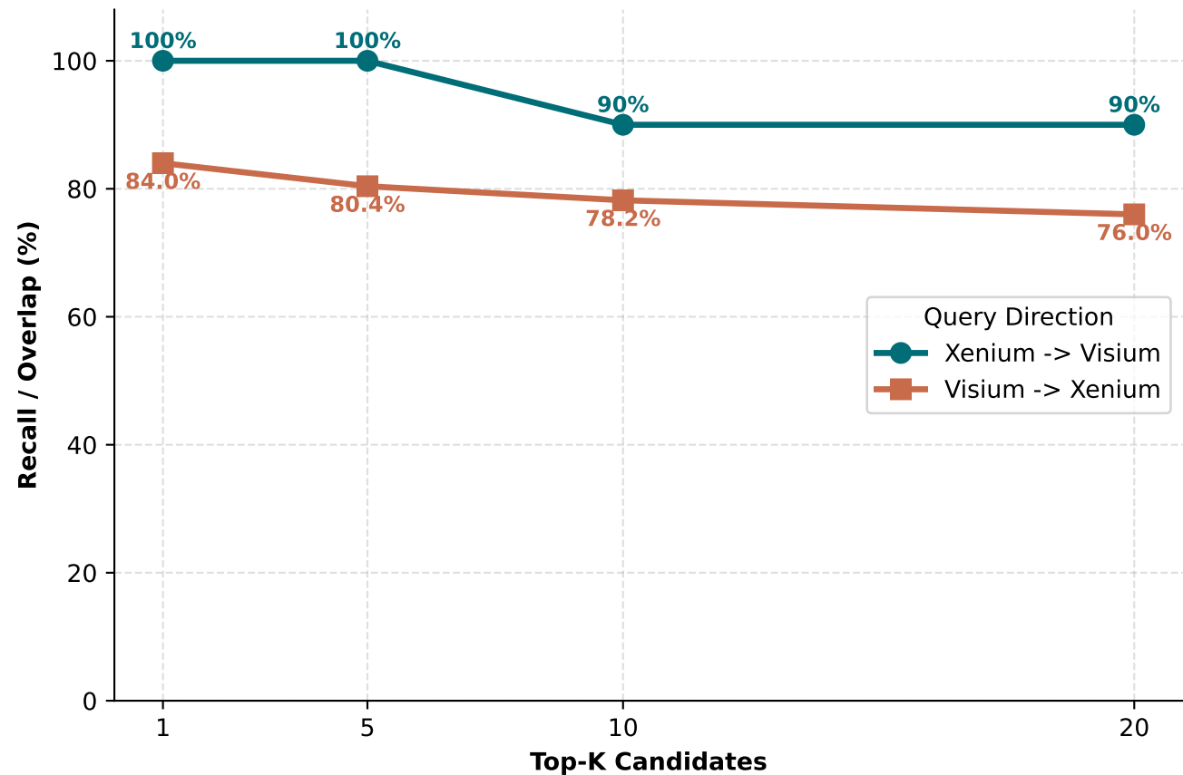
Cross-Modality Retrieval Accuracy (Recall vs Top-K)
