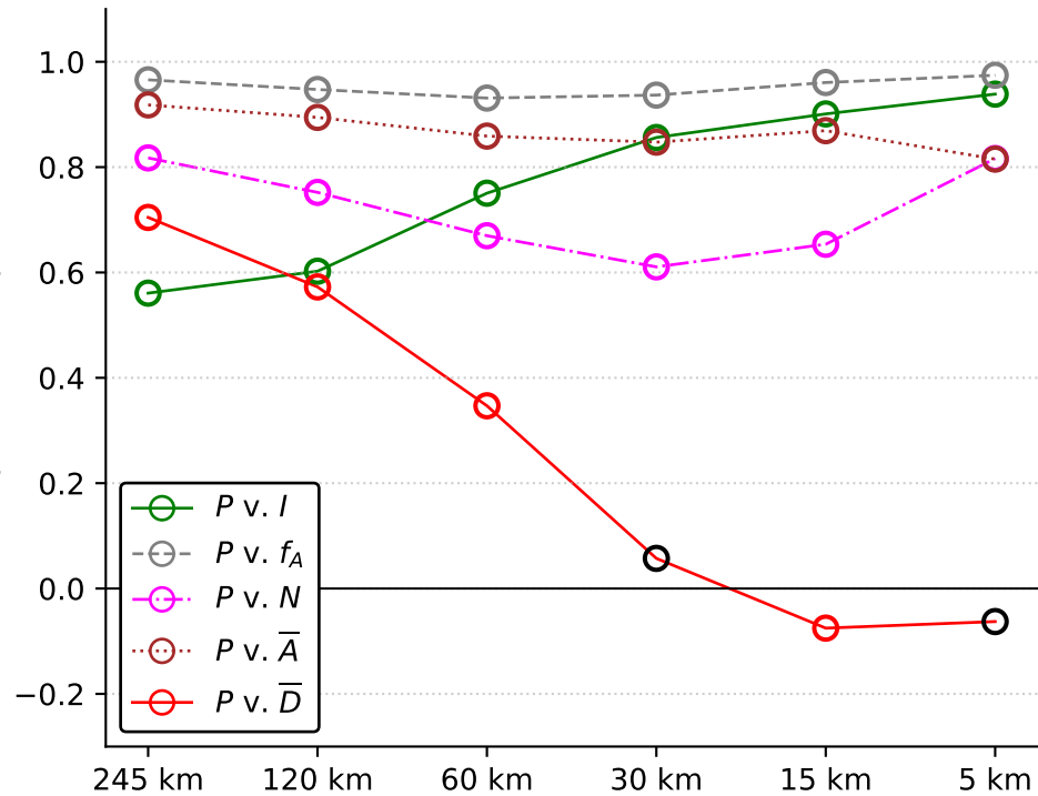
Spearman's \rho
