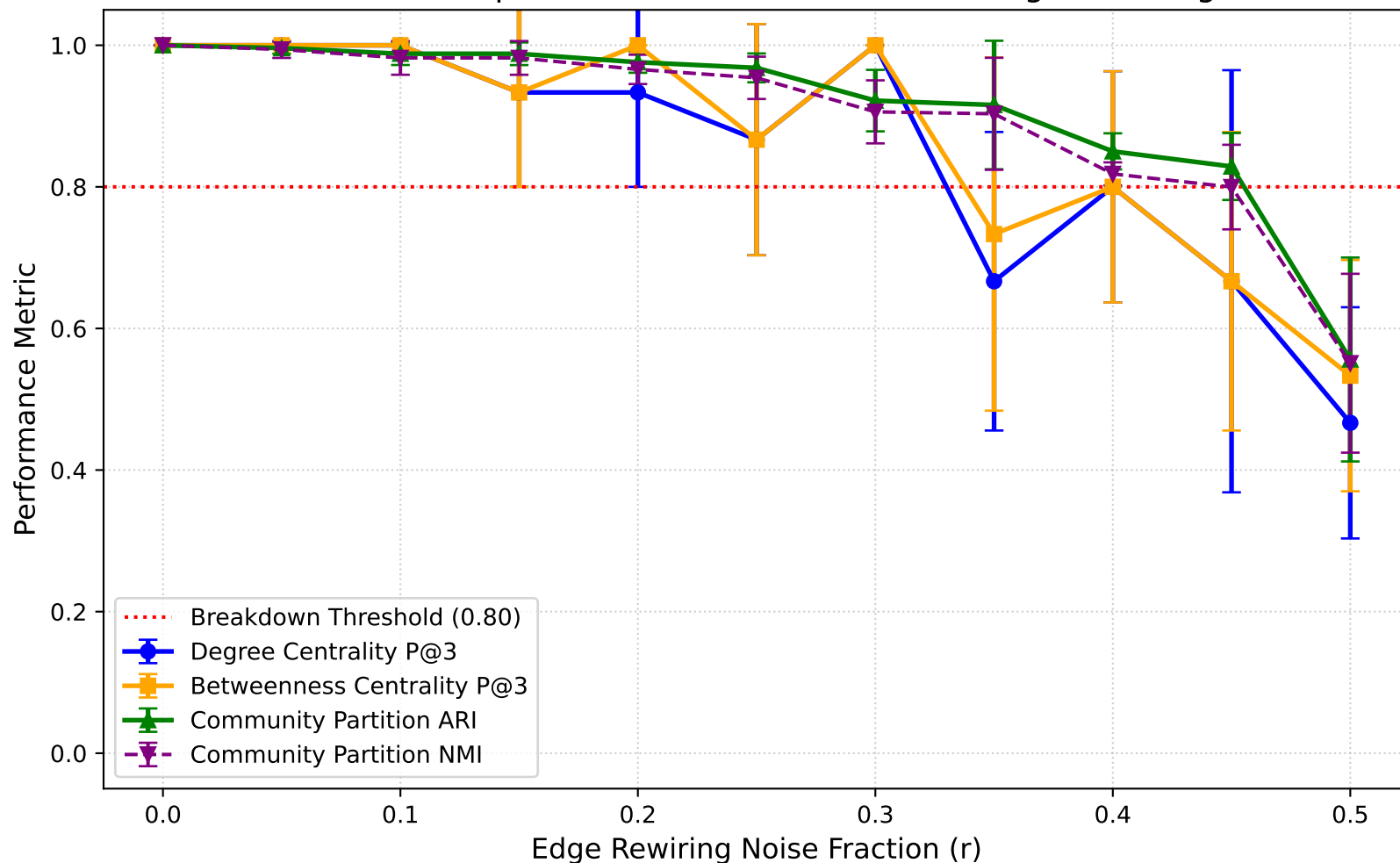
Robustness of Graph Methods under Controlled Edge Rewiring Noise
