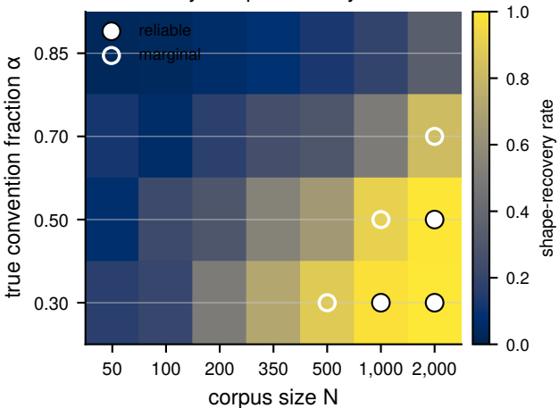
Reachability: shape recovery over N \times \alpha
