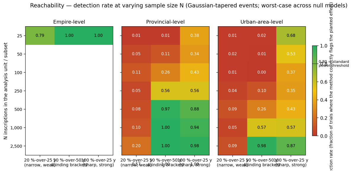
Figure 6: Detection rate by sample-size N (rows) × effect bracket (columns). Each panel = an analysis level. Worst-case across null models. Green 0.80 (reliably reachable); yellow partial; red unreachable. Gaussian-tapered events.
