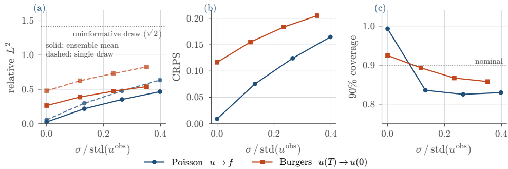
Fig. 10. Noise sweeps on both inverse problems, against noise measured in units of the observation’s own standard deviation so the two benchmarks share an axis. (a) Relative L^2 : the ensemble mean (solid) beats a single draw (dashed) by 1.35\text{--}2.3\times everywhere, and no cell reaches the uninformative level of Remark 8. (b) CRPS. (c) 90% coverage: the clean Poisson cell is the outlier, and it is the one whose posterior is nearly a Dirac.
