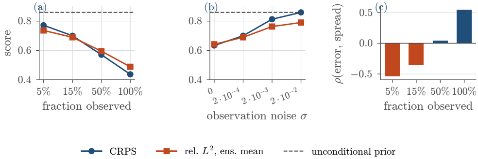
Fig. 9. Inverse Darcy, \kappa target, as the observation is degraded. (a) Observed fraction at \sigma = 2 \times 10^{-4} . (b) Noise at 15% observed. In both, the dashed line is the unconditional model: a curve reaching it is a model that has stopped using its data. (c) Rank correlation between per-sample ensemble spread and per-sample error, which changes sign across the sweep.
