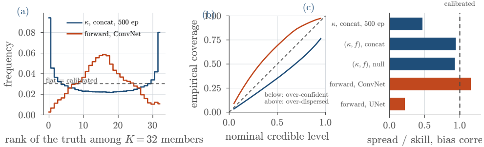
Fig. 7. Calibration, K = 32 . (a) Rank histograms: the inverse model U-shaped (under-dispersed), the forward one dome-shaped. (b) Reliability against the diagonal. (c) Bias-corrected spread-skill; the two forward models, whose true posterior is identical and degenerate, disagree by a factor of five.
