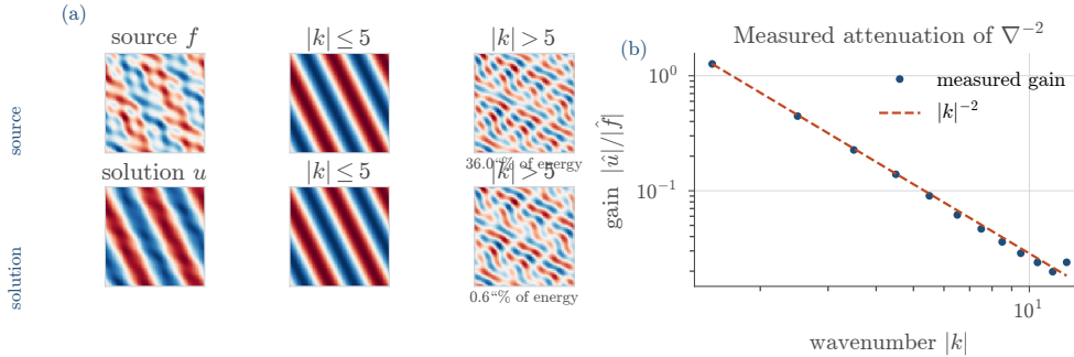
Fig. 3. (a) A Poisson source and solution split at |k| = 5 : above the cut sits 36% of the source’s energy and 0.6% of the solution’s. (b) Measured spectral gain against |k|^{-2} . Both use a widened source, since the generator’s default carries no energy above |k| = 3 — itself a reason to distrust errors measured on it.
