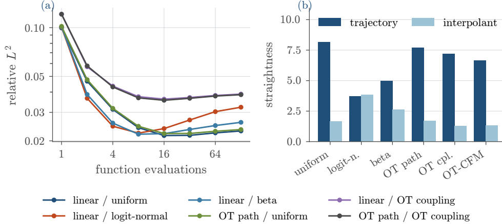
Fig. 6. (a) Error against function evaluations, Euler, averaged over three seeds. The curves cross: the configuration that wins below eight evaluations loses above sixteen. (b) The two straightness definitions disagree about which configuration is straight, and only the trajectory one predicts (a).
