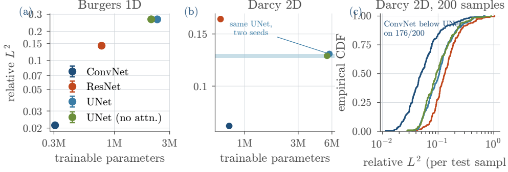
Fig. 4. (a, b) Accuracy against parameters; the ordering is inverted with respect to capacity. Error bars in (a) are the standard deviation over three matched seeds, and are smaller than the markers. The band in (b) spans two runs of the identical UNet at different seeds — the only replicate available on Darcy. (c) Per-sample errors on Darcy.
