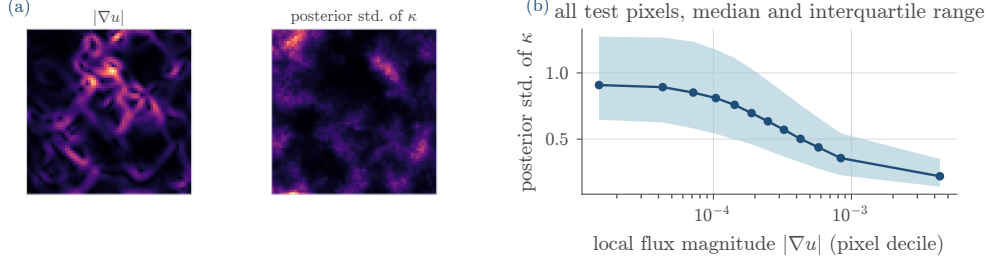
Fig. 8. Spatially varying identifiability. (a) |\nabla u| and the posterior standard deviation of \kappa for one condition; the bright regions coincide. (b) All test pixels by flux decile: posterior width falls 3.9\times from lowest to highest.
