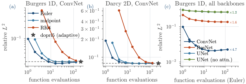
Fig. 5. Accuracy against cost on frozen weights. (a, b) The best backbone per problem; the star and dashed line mark the converged solution of the learned ODE. (c) Euler on every Burgers backbone. The slope is the diagnostic: steep means discretization error dominates, flat means the field is the limitation.
