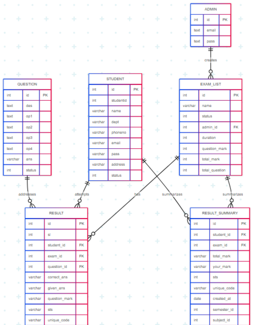
Figure 3.2: E-R Diagram.
