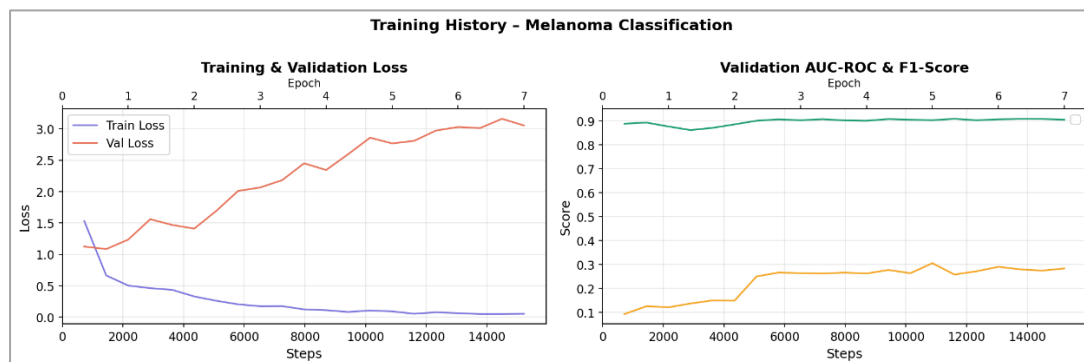
Figure 2: Training and validation loss (left) and validation AUC-ROC & F1-Score (right) over epochs for the multimodal model.
