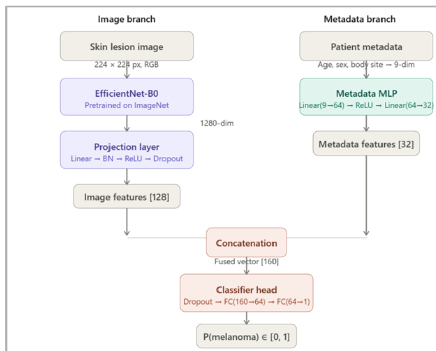
Figure 1: Multimodal model architecture
