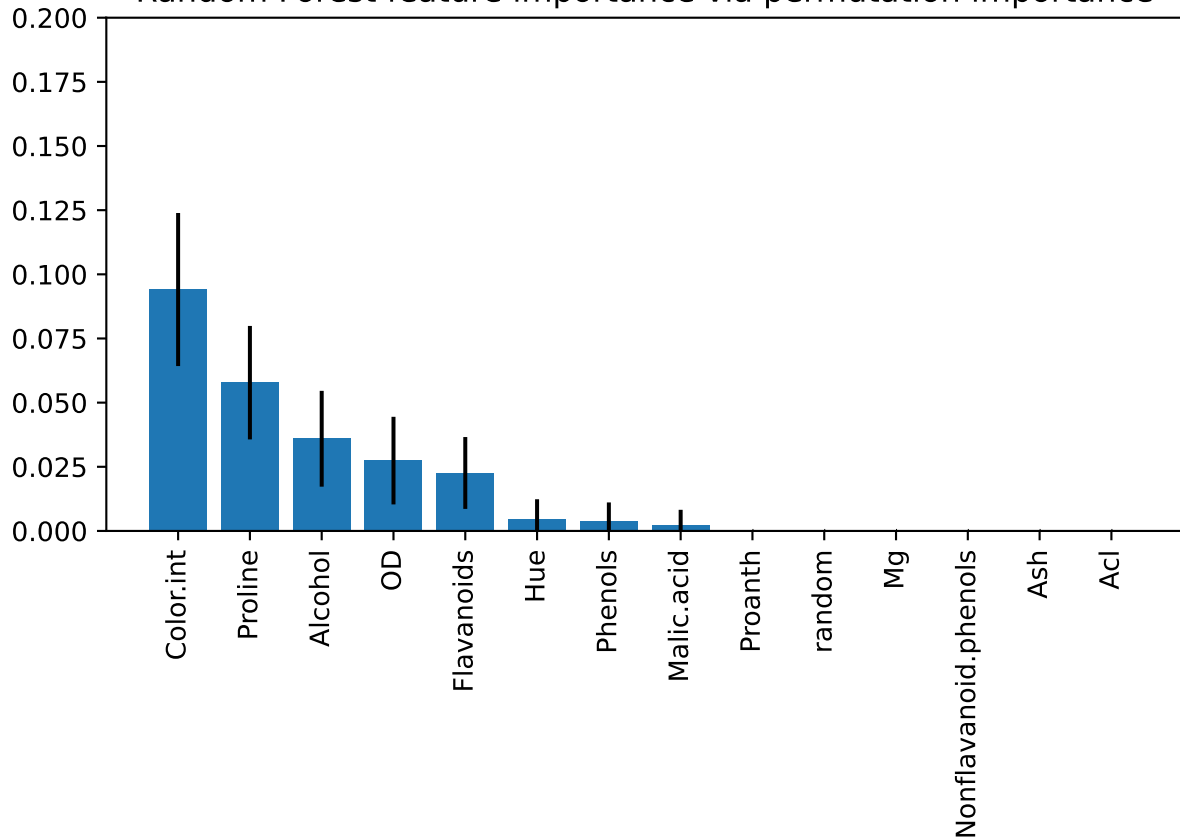
Random Forest feature importance via permutation importance
