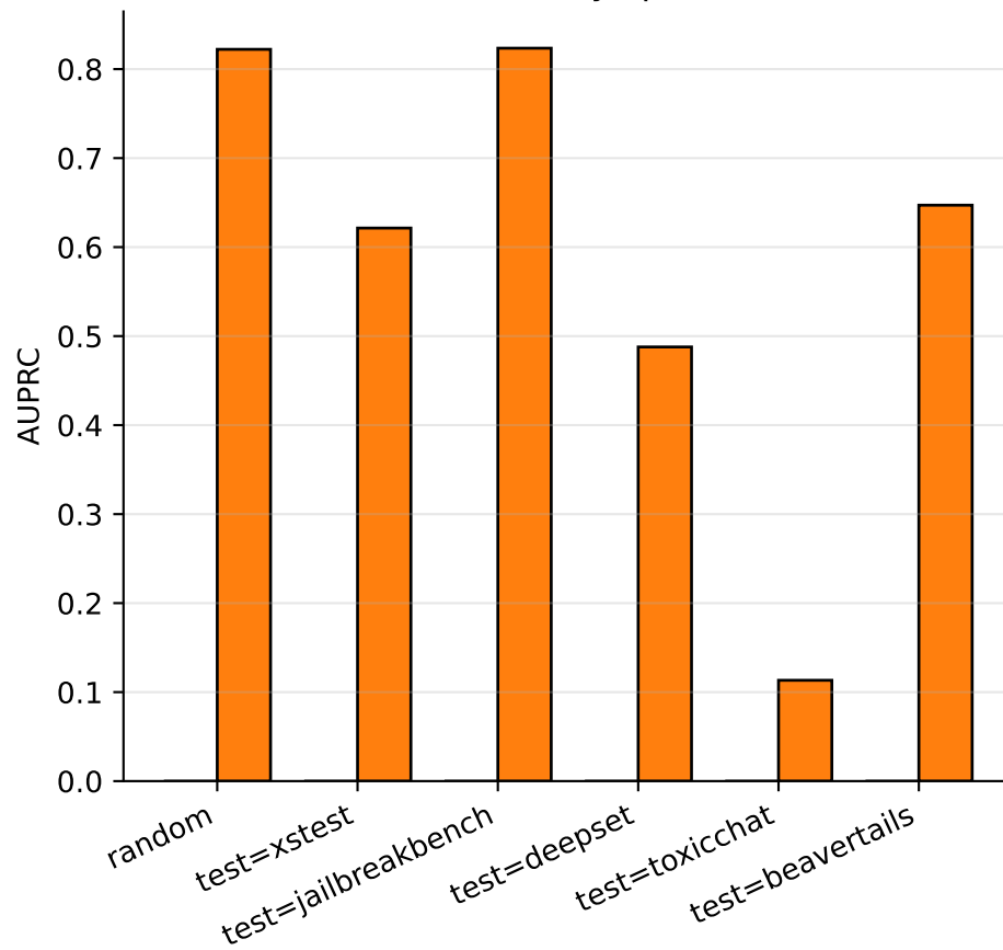
AUPRC by split
