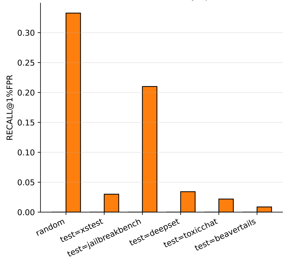
RECALL@1%FPR by split
