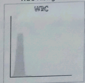
WBC Histogram
