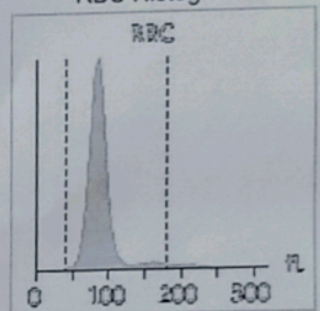
RBC Histogram
