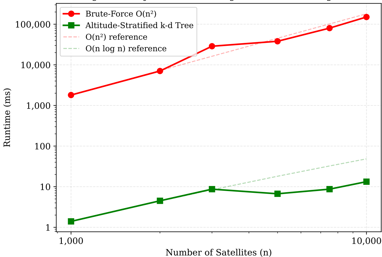
Fig. 1 — Conjunction Screening Runtime vs Catalog Size
