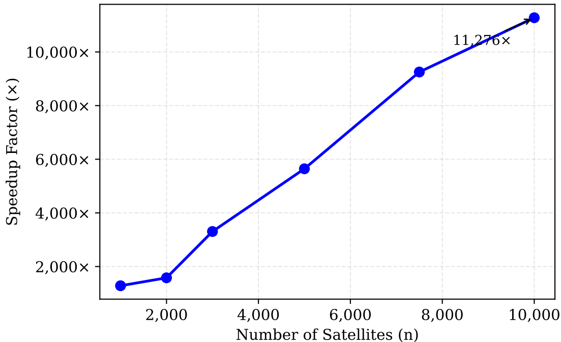
Fig. 2 — k-d Tree Speedup over Brute-Force
