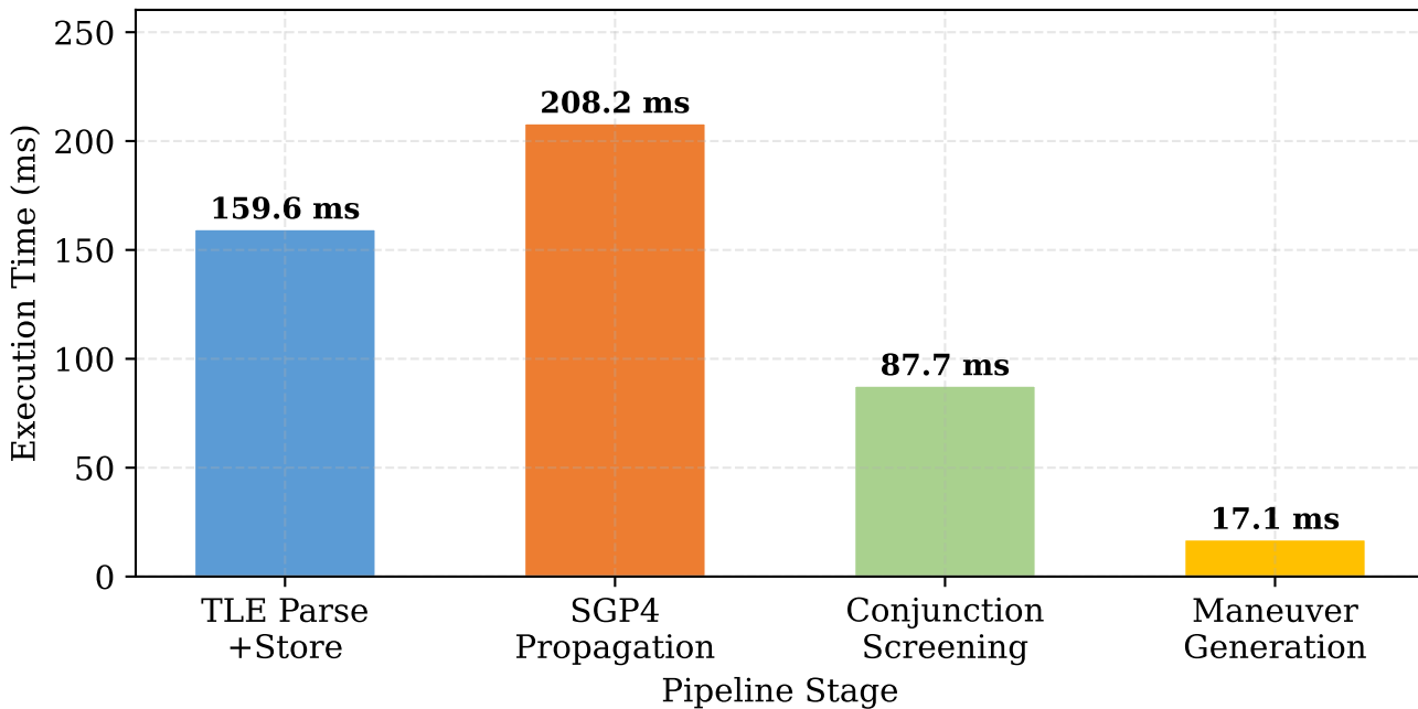
Fig. 4 — Pipeline Stage Latency Breakdown (n=10,303 satellites, total=472.6 ms, network excluded)
