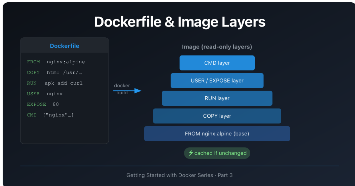
Figure 4: Dockerfile and Building Custom Images
