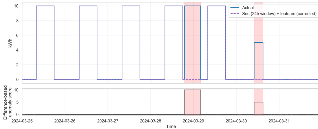
Figure 4.4: The same 24-hour window model from Figure 4.1, but applied with inference-time imputation. When an anomaly is detected, the predicted value replaces the actual value in the sliding window for future steps. This prevents error propagation and maintains a high anomaly score throughout the event.
