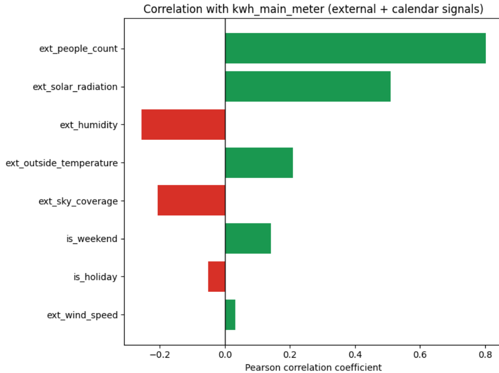
Figure 5.1: Empirical Pearson correlation of contextual and external drivers with the main electricity meter over the synthetic 2007 benchmark year.
