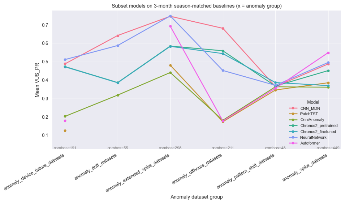
Figure 5.5: Chronos-2 vs. CNN_MDN under season-matched three-month baselines.
