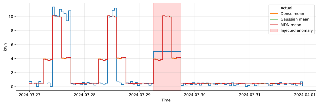
Figure 4.5: Predicted means over the Variable Shift horizon. Dense, Gaussian, and MDN models track the two regimes, masking the scoring deficiencies discussed in Sections 4.7.1–4.7.3.
