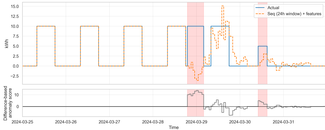
Figure 4.1: Prediction behavior of a model using a 24 h historical window plus time features. The top panel shows actual vs. predicted values; the bottom panel shows the difference-based anomaly score. Note the erratic predictions even after the anomaly ends as the unseen data propagates through the sliding window.
