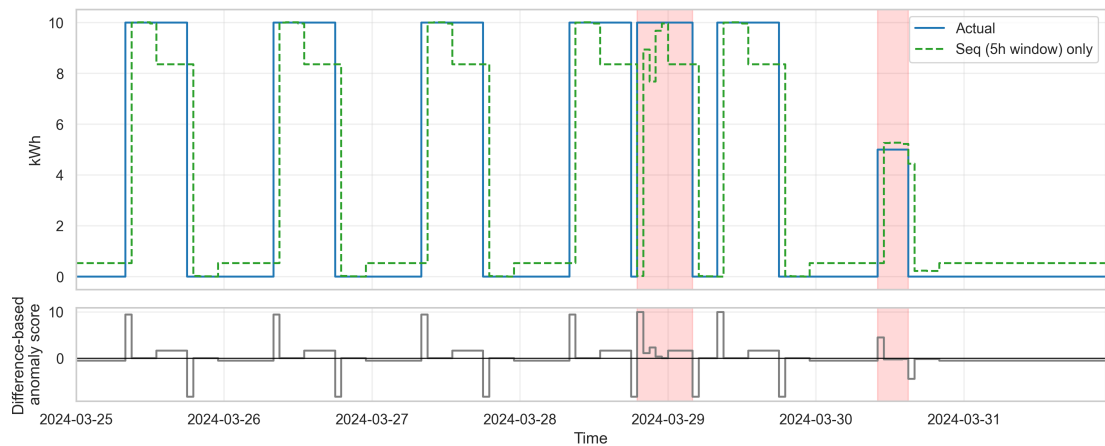
Figure 4.2: Prediction behavior of a model using only a short (5-step) historical window. The model correctly identifies the onset of anomalies but rapidly adapts to the new level, causing the anomaly score to drop back to near zero while the anomaly is still ongoing.
