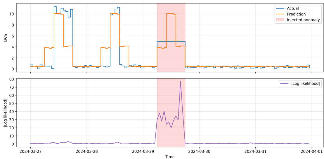
Figure 4.9: MDN absolute log-likelihood trace. The stuck-at-5 anomaly triggers a sustained spike because the value resides in a low-probability region between mixture components.
