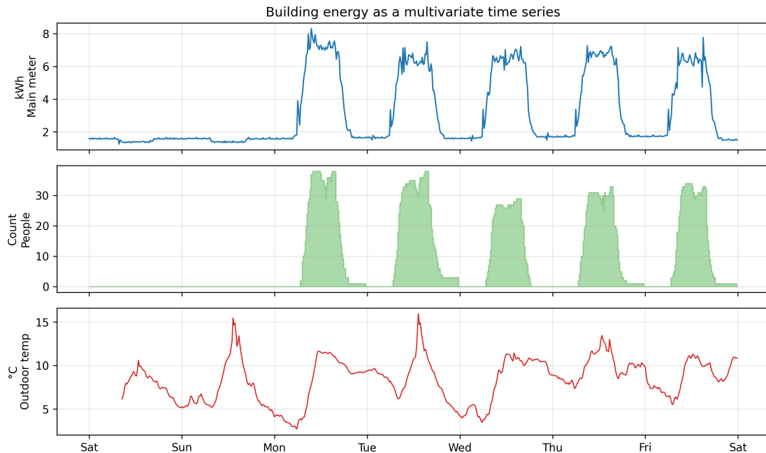
Figure 2.1: Representative multivariate time series showing the main meter load together with occupancy (people count) and outdoor temperature. The plot illustrates how multiple interdependent variables evolve jointly over time.
