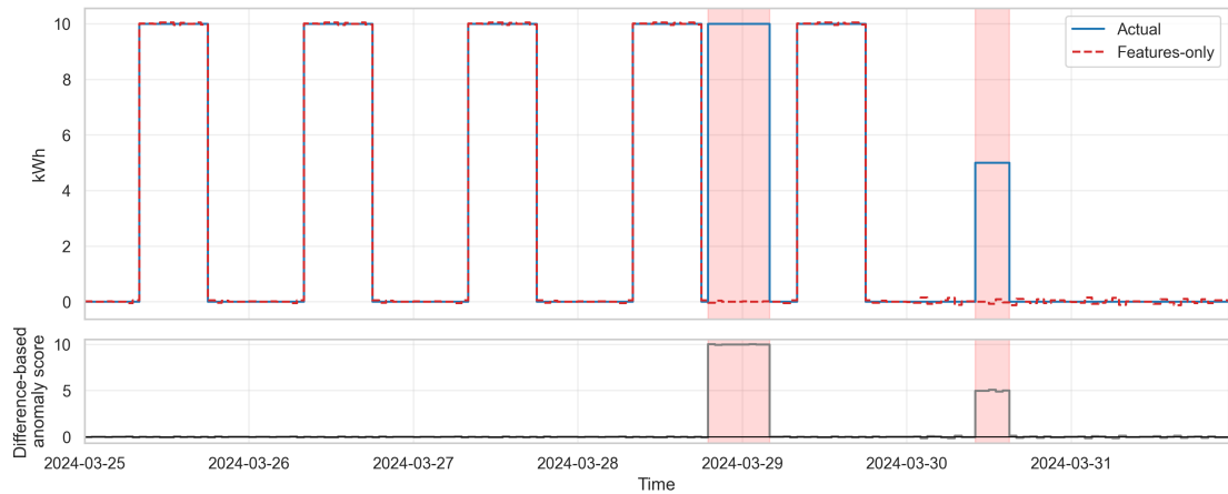
Figure 4.3: Behavior of a features-only model (no historical consumption input). The prediction relies solely on context (time/weekend), resulting in a stable baseline and accurate detection of sustained anomalies without adaptation.
