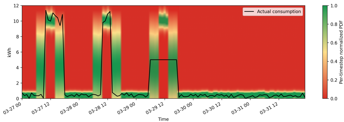
Figure 4.8: Per-timestep normalized PDF for the Gaussian model. High probability mass accumulates between the actual clusters, illustrating the variance-stretching paradox.
