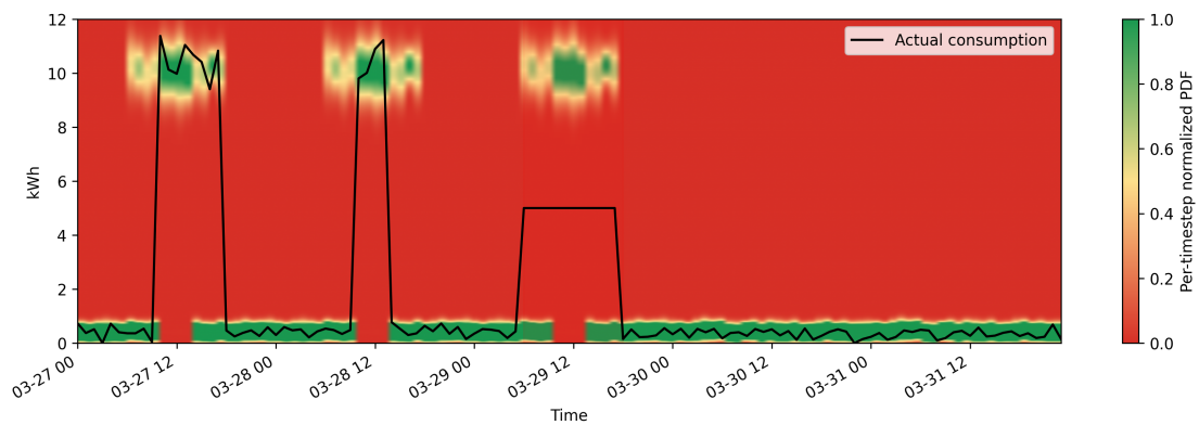
Figure 4.10: MDN normalized PDF heatmap. Two distinct high-probability ridges align with the real operating modes, while the middle band remains improbable.
