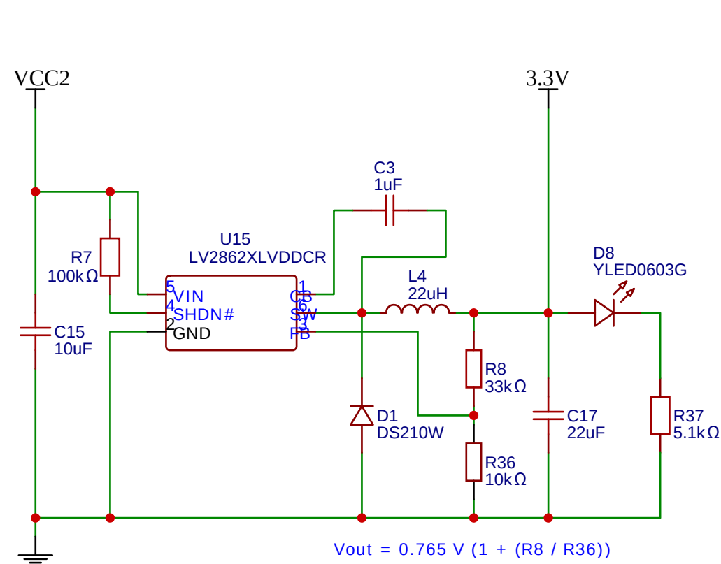
Power Supply 3.3V/0.6A
