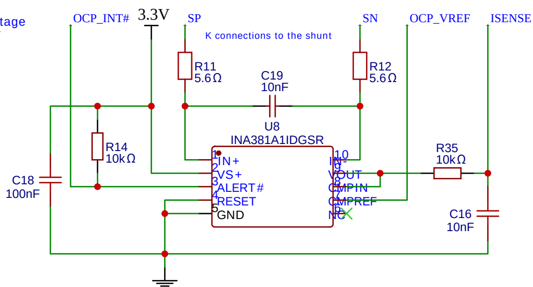
Input OCP 20x current amplifier with comparator 0.004R shunt = 1A/80mV - 40A/3200mV Input filter R11, R12 and C19 Output filter R35/C16 for the MCU ADC
