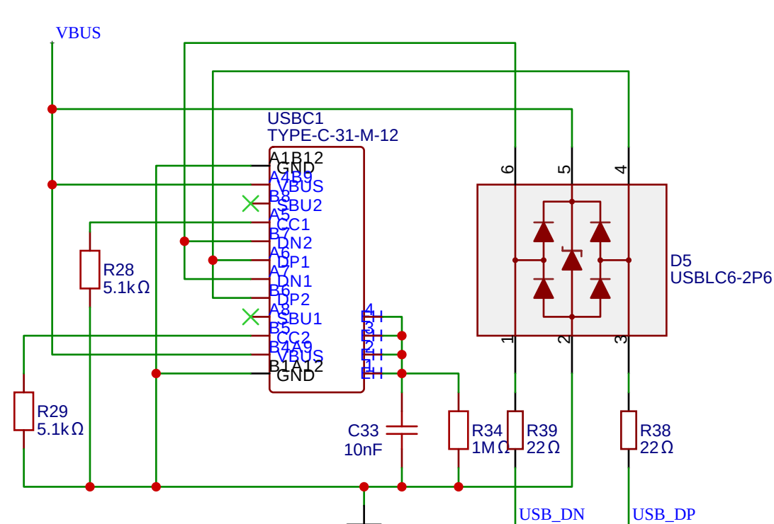
USB connector for programming
