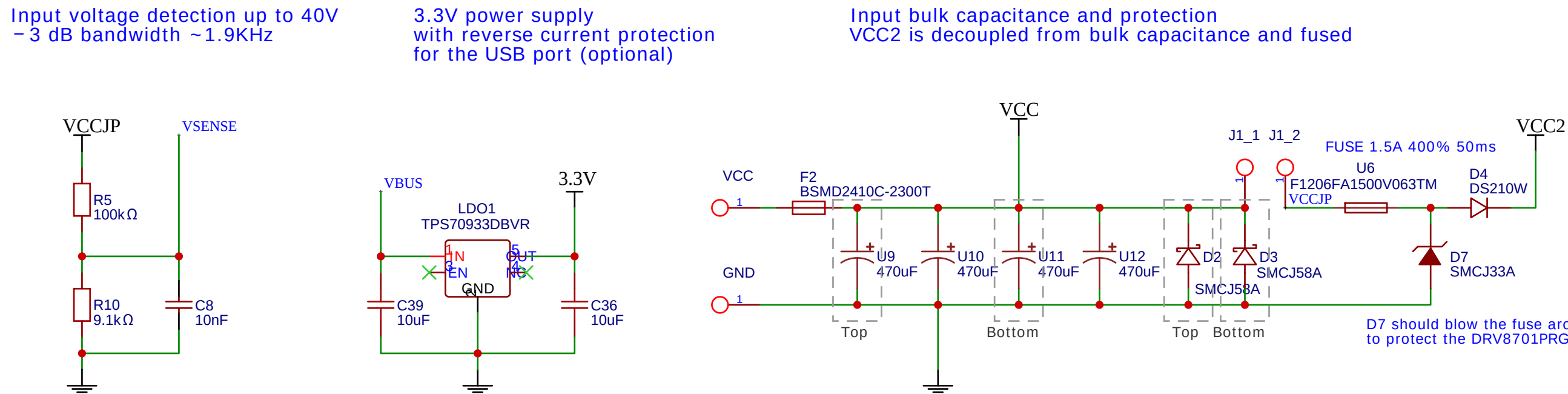
Power Supply 3.3V/0.6A
