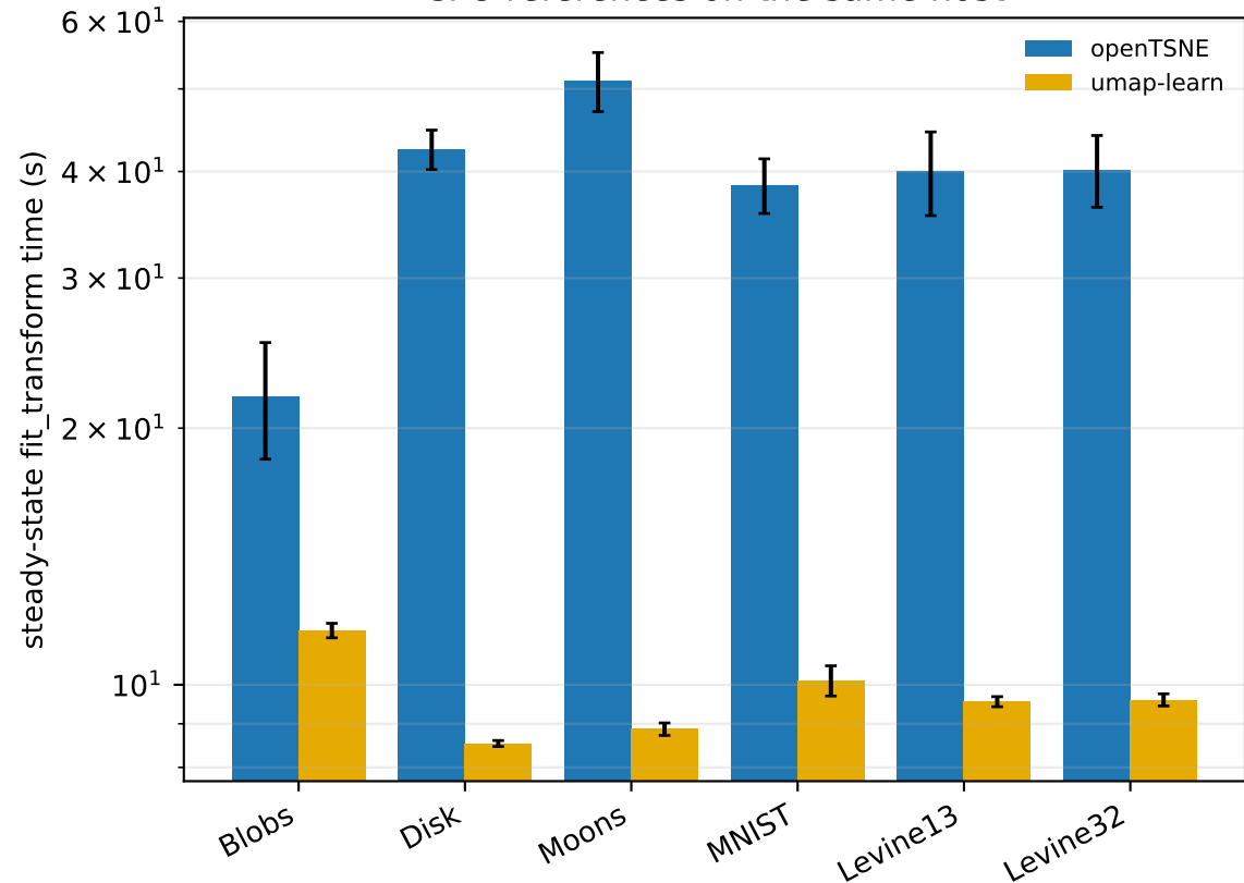
CPU references on the same host
