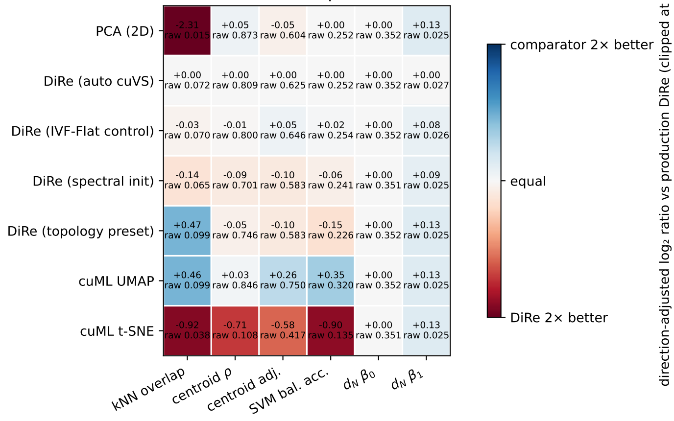
Large-data fidelity versus production DiRe (centroid effect uses (1+p)/2 ; cells retain row p )
