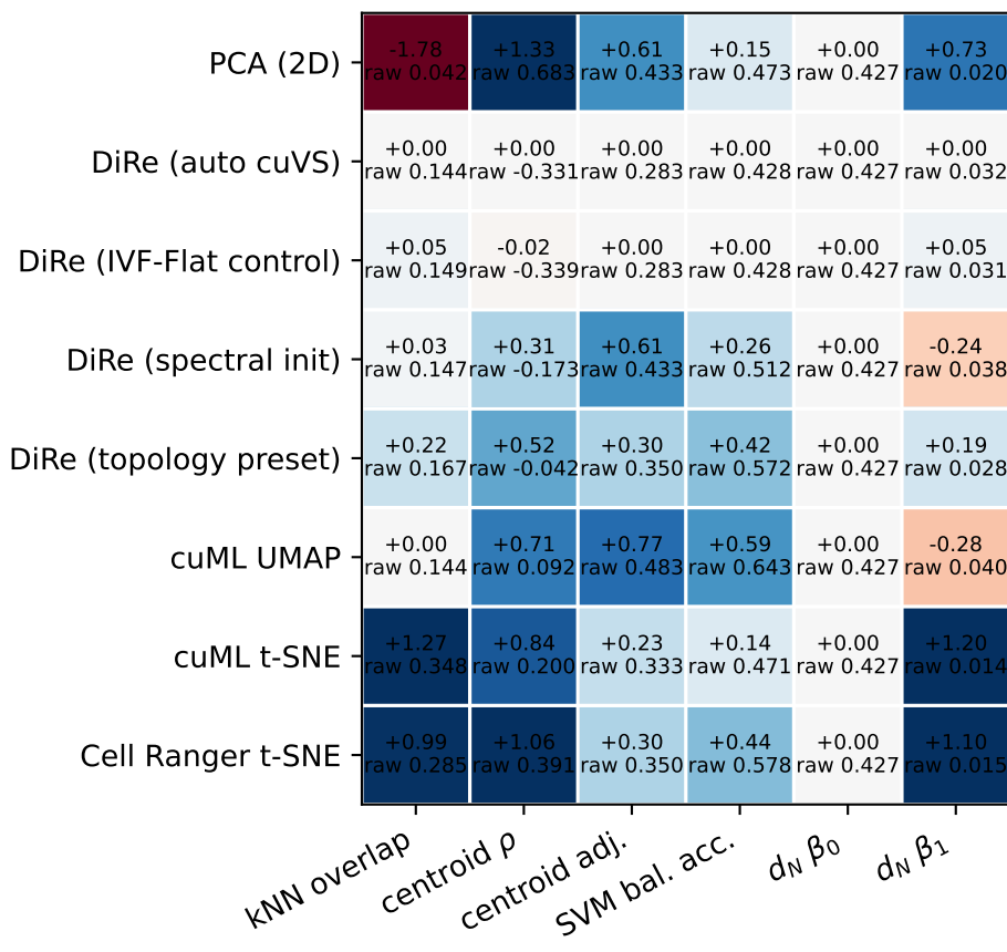
Large-data fidelity versus production DiRe (centroid effect uses (1+p)/2 ; cells retain row p )
