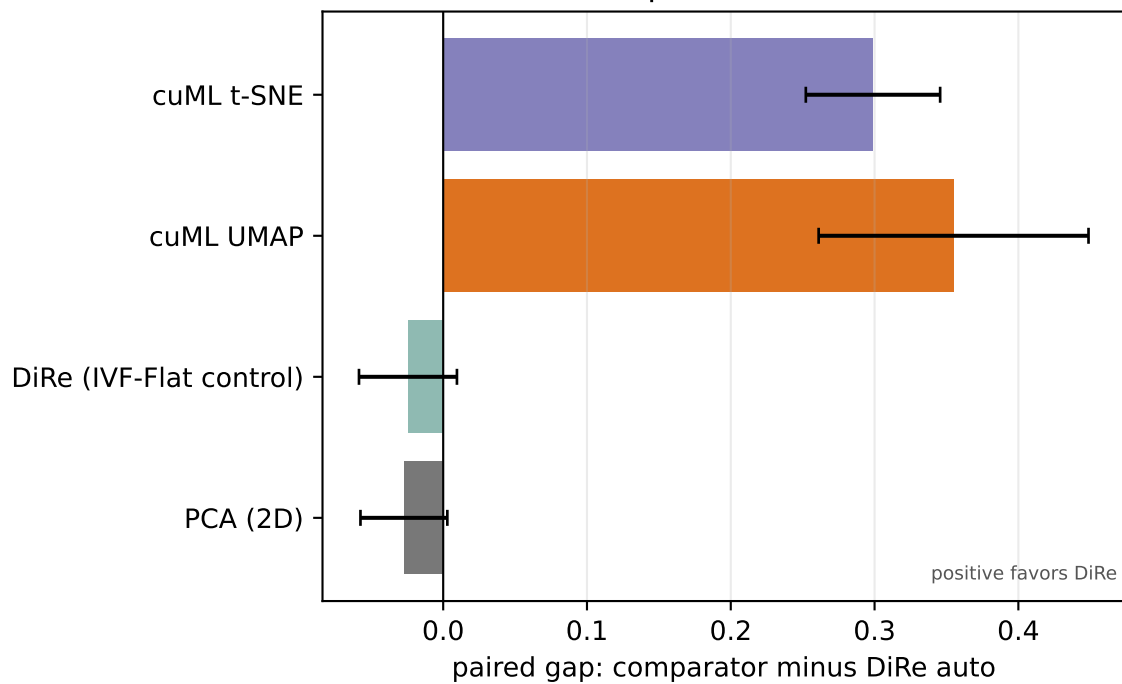
arXiv corpus: H1 Betti-DTW
