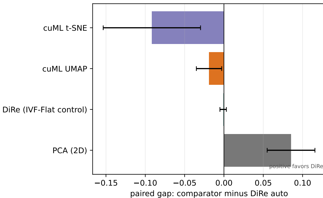
arXiv corpus: H0 Betti-DTW
