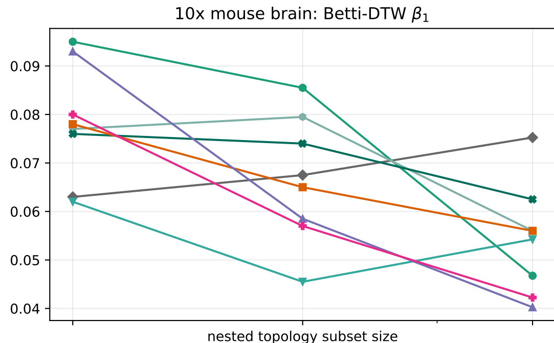
Betti-DTW subset-size sensitivity on fixed full-data layouts
