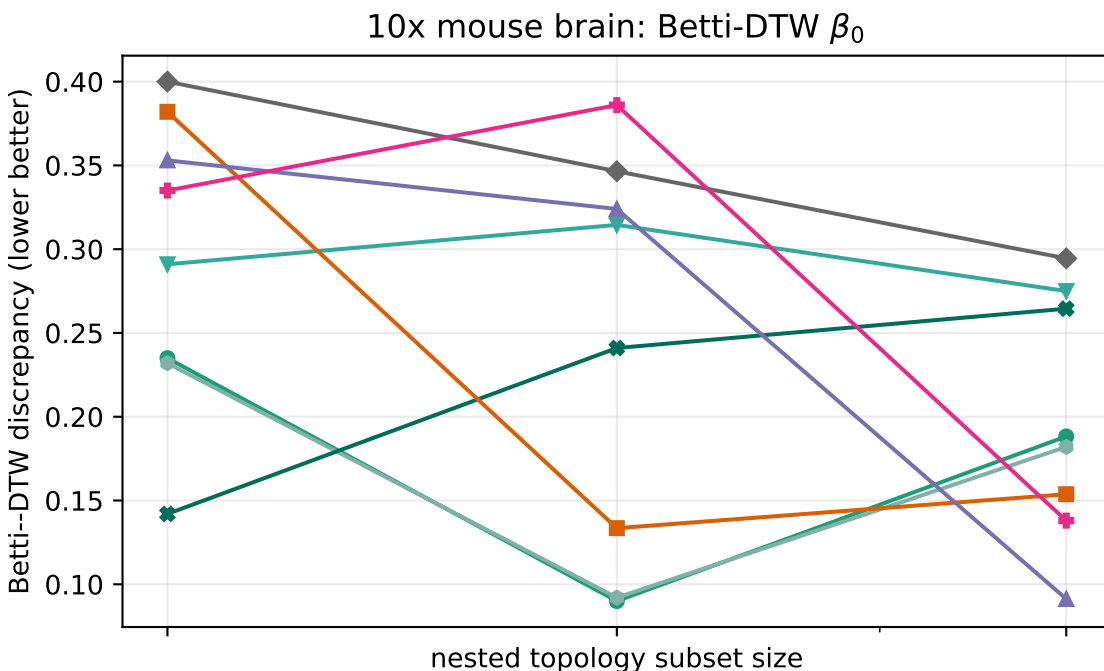
Betti-DTW subset-size sensitivity on fixed full-data layouts
