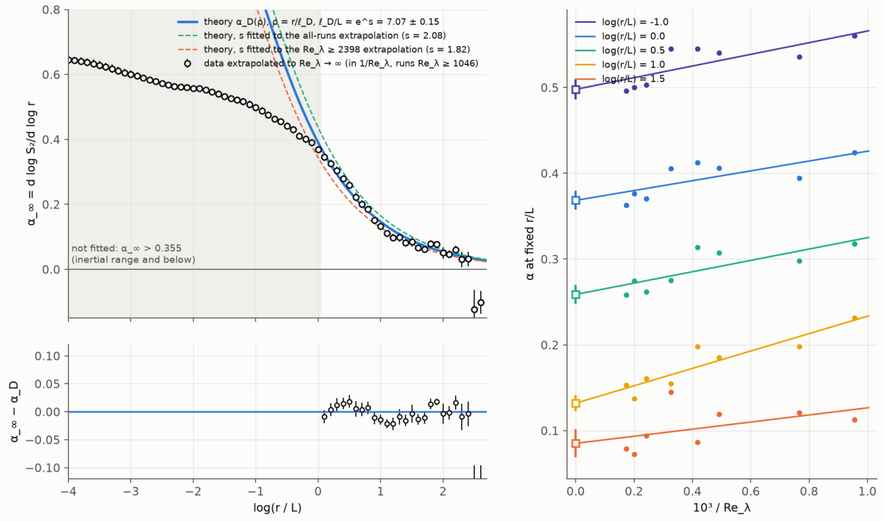
FIG. 9. Left: the Max Planck index extrapolated to Re_{\lambda} \rightarrow \infty in 1/Re_{\lambda} (circles, runs Re_{\lambda} \geq 1046 ) against the odd-ensemble theory with one scale parameter (blue). Dashed lines use the shifts fitted to the extrapolations with all runs and with Re_{\lambda} \geq 2398 only. The fit uses the tail outside the shaded region; the residuals are shown below. Right: \alpha_{\text{exp}} against 1/Re_{\lambda} at fixed r/L ; squares are the extrapolated values.
