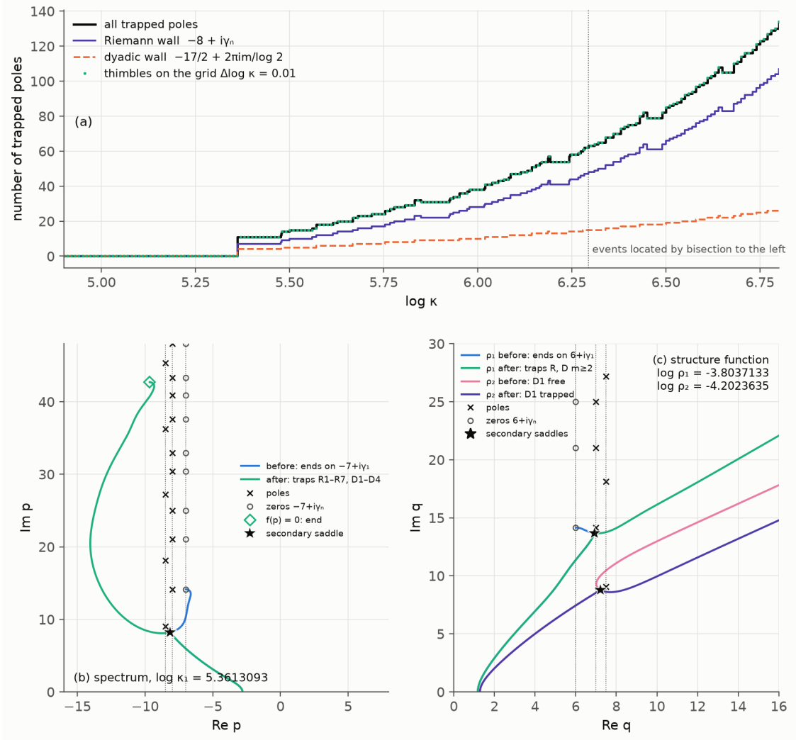
FIG. 6. (a) Stokes staircase of the energy spectrum in the odd Euler ensemble: the numbers of trapped Riemann-wall and dyadic-wall poles and their total, from the 49 Stokes events located by bisection for \log \kappa \leq 6.3 (dotted line) and from the thimbles on a grid of step 0.01 (dots; they are followed to t = 20 , where the integrand has fallen by e^{-400} ). Each trapped pole adds a log-periodic correction to H(\kappa) . (b) The thimbles at the two ends of the bisection bracket of the first event, 10^{-8} apart. Before it the thimble ends on the zero -7 + i\gamma_1 ; after it, past the secondary saddle (star), it traps P_1-P_7 and D_1-D_4 and ends on a zero of f(p) (diamond). (c) The same for the two events of the structure function.
