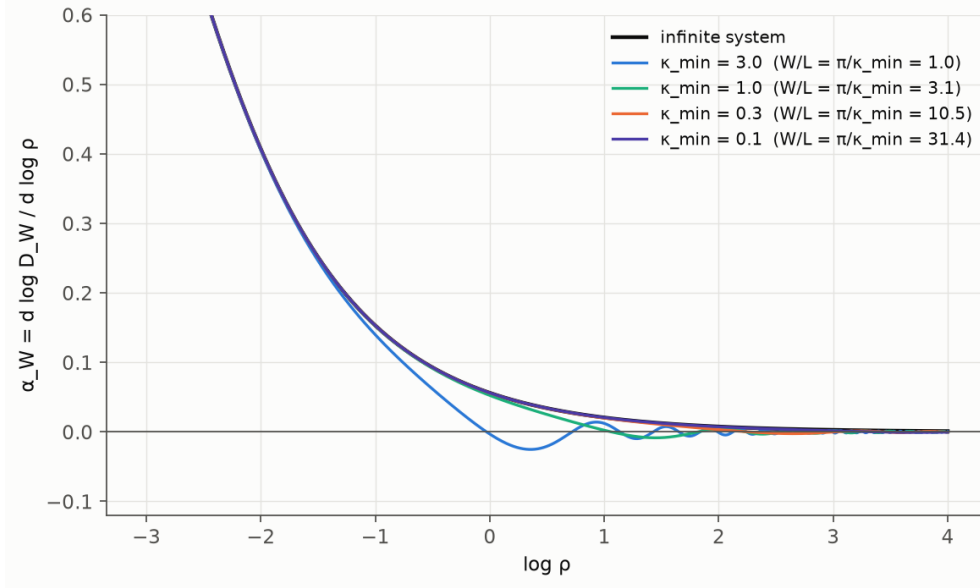
FIG. 7. The effective index of the finite system, Eq. (18), for several infrared cutoffs \kappa_{\min} = \pi L/W , compared with the infinite system.
