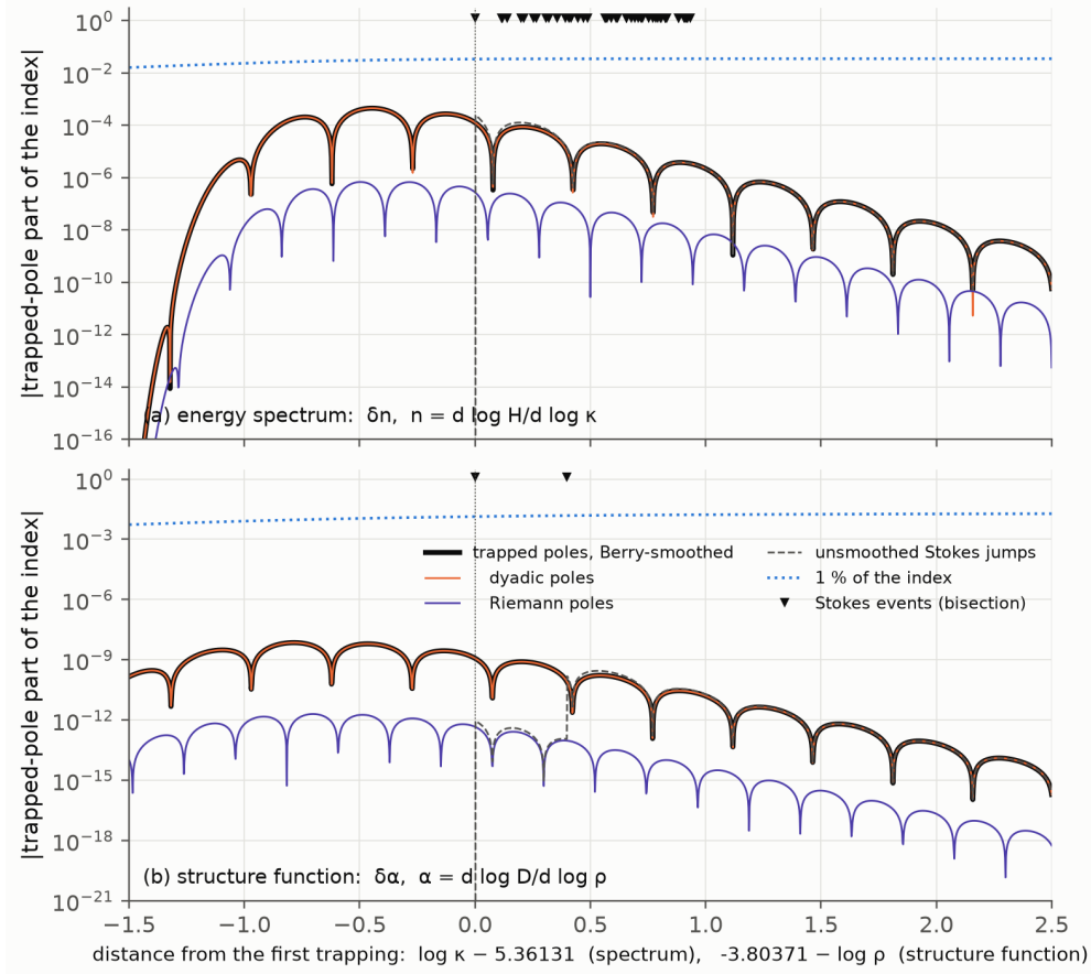
FIG. 5. Trapped-pole (log-periodic) part of the local index, Eq. (17): Berry-smoothed (thick black), its dyadic (orange) and Riemann (violet) parts, and the unsmoothed Stokes jumps (dashed), against the distance from the first trapping. (a) The energy spectrum, \delta n , n = d \log H/d \log \kappa , from \log \kappa_1 = 5.36131 . (b) The structure function, \delta \alpha , from \log \rho_1 = -3.80371 . Triangles mark the Stokes events, the dotted line 1% of the index.
