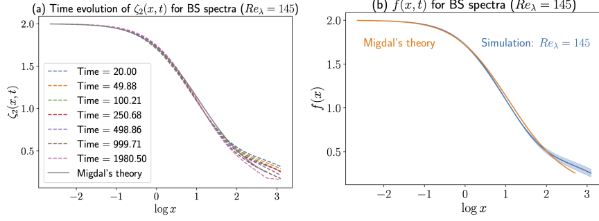
FIG. 10. Effective index \langle r \partial_r \log(\Delta v^2) \rangle of the 4096^3 DNS of decaying turbulence by Rodhiya and Sreenivasan [13] (Birkhoff–Saffman initial spectrum) against the Euler-ensemble prediction (from Ref. [6]).
